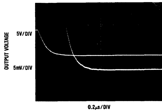
Settling Time
