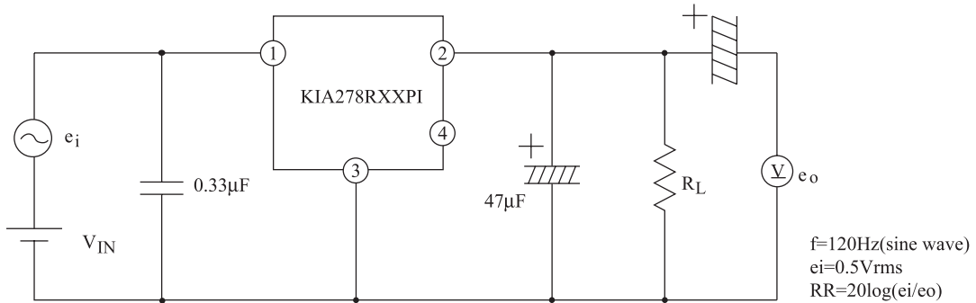
Fig. 1-2 Ripple Rejection Test Circuit
