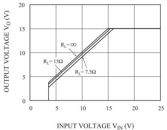
Fig.6-5 V_{IN} - V_O (KIA278R15)
