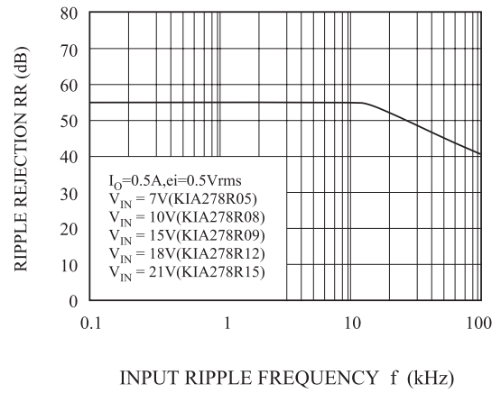
Fig. 10-1 f - RR
