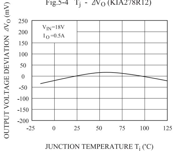
Fig.5-4 T_j - \Delta V_O (KIA278R12)
