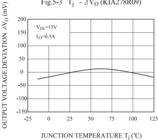
Fig.5-3 T_j - \Delta V_O (KIA278R09)
