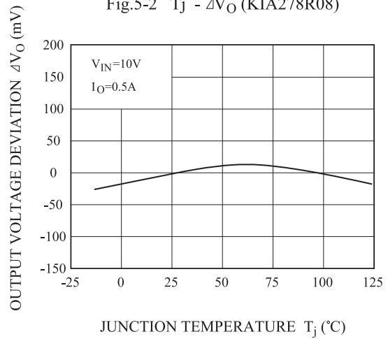
Fig.5-2 T_j - \Delta V_O (KIA278R08)
