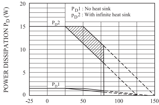
Fig.3 T_a - P_D
