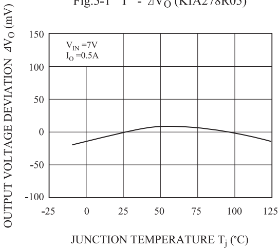
Fig.5-1 T_j - \Delta V_O (KIA278R05)
