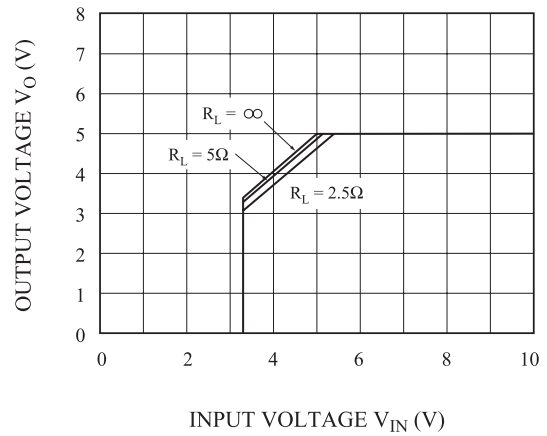
Fig.6-1 T_j - V_O (KIA278R05)
