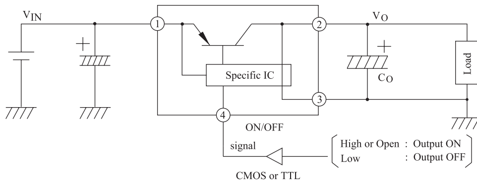
Fig. 2 Application Circuit for Standard
