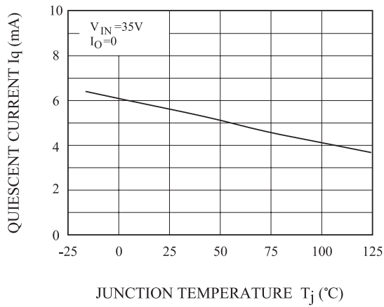
Fig.9 T_j - I_q
