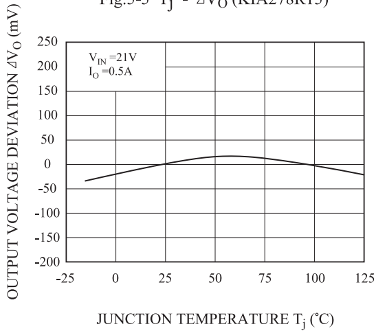
Fig.5-5 T_j - \Delta V_O (KIA278R15)
