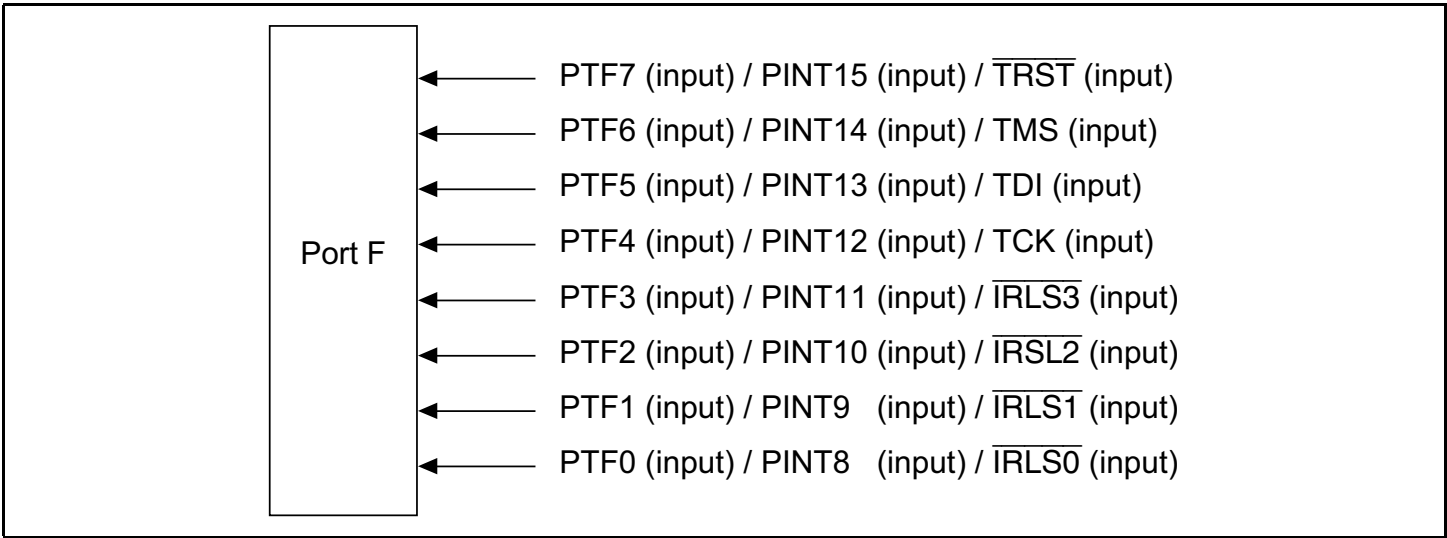
Figure 19.6 Port F
