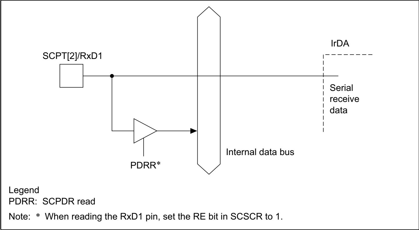
Figure 17.4 SCPT[2]/RxD1 Pin
