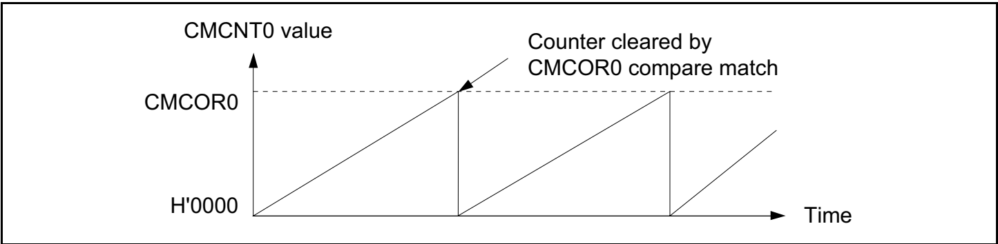
Figure 11.25 Counter Operation
