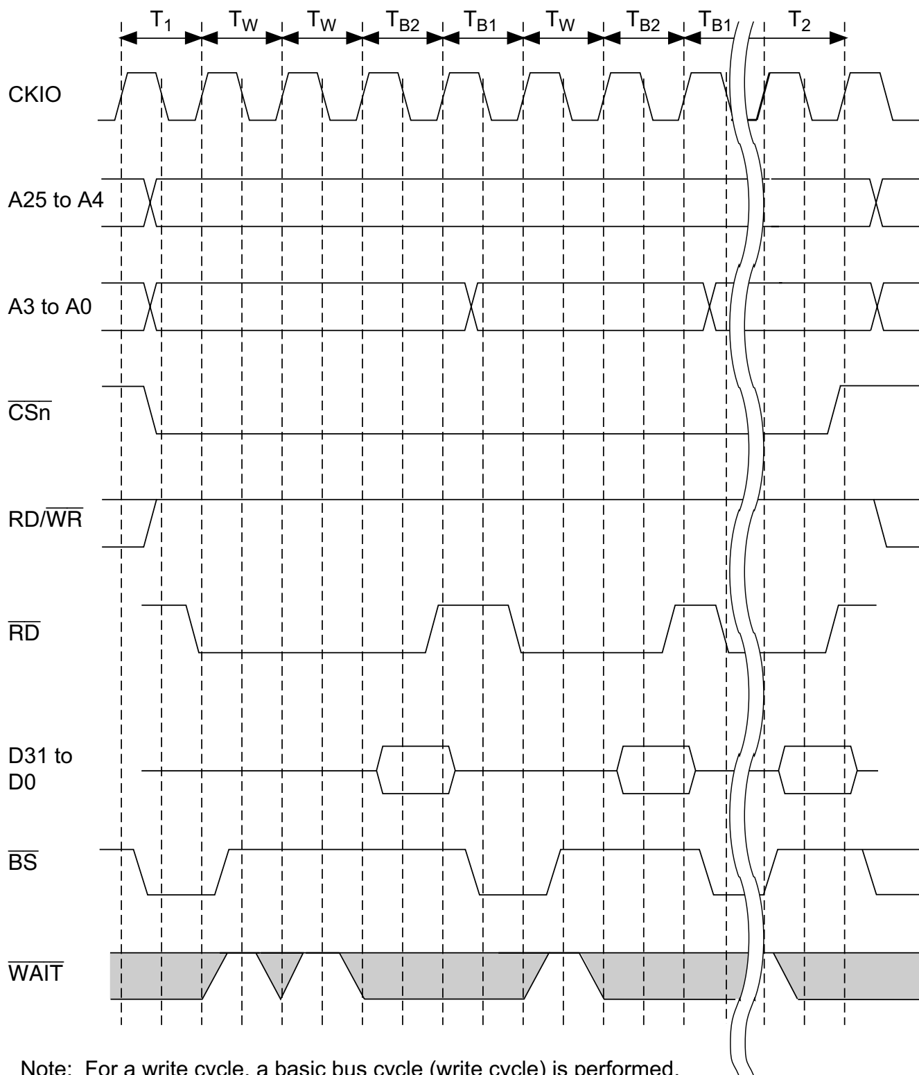
Figure 10.29 Burst ROM Wait Access Timing
