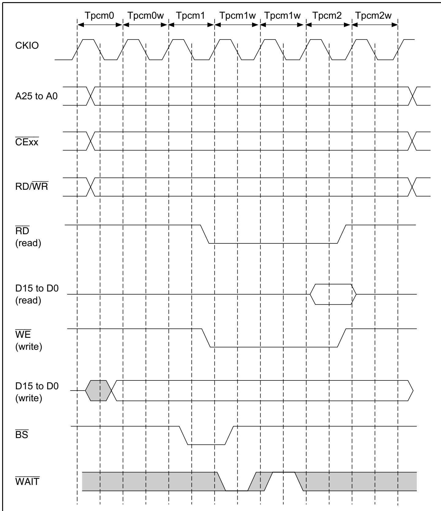
Figure 10.33 Wait Timing for PCMCIA Memory Card Interface
