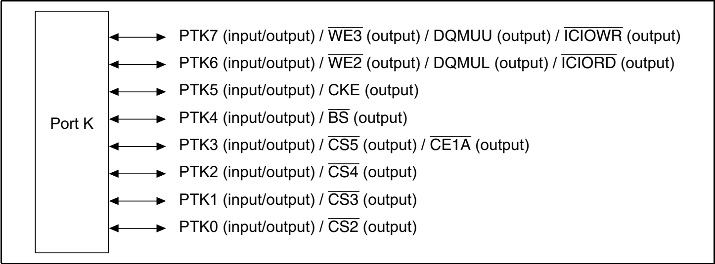
Figure 19.10 Port K
