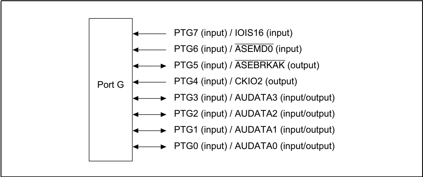
Figure 19.7 Port G
