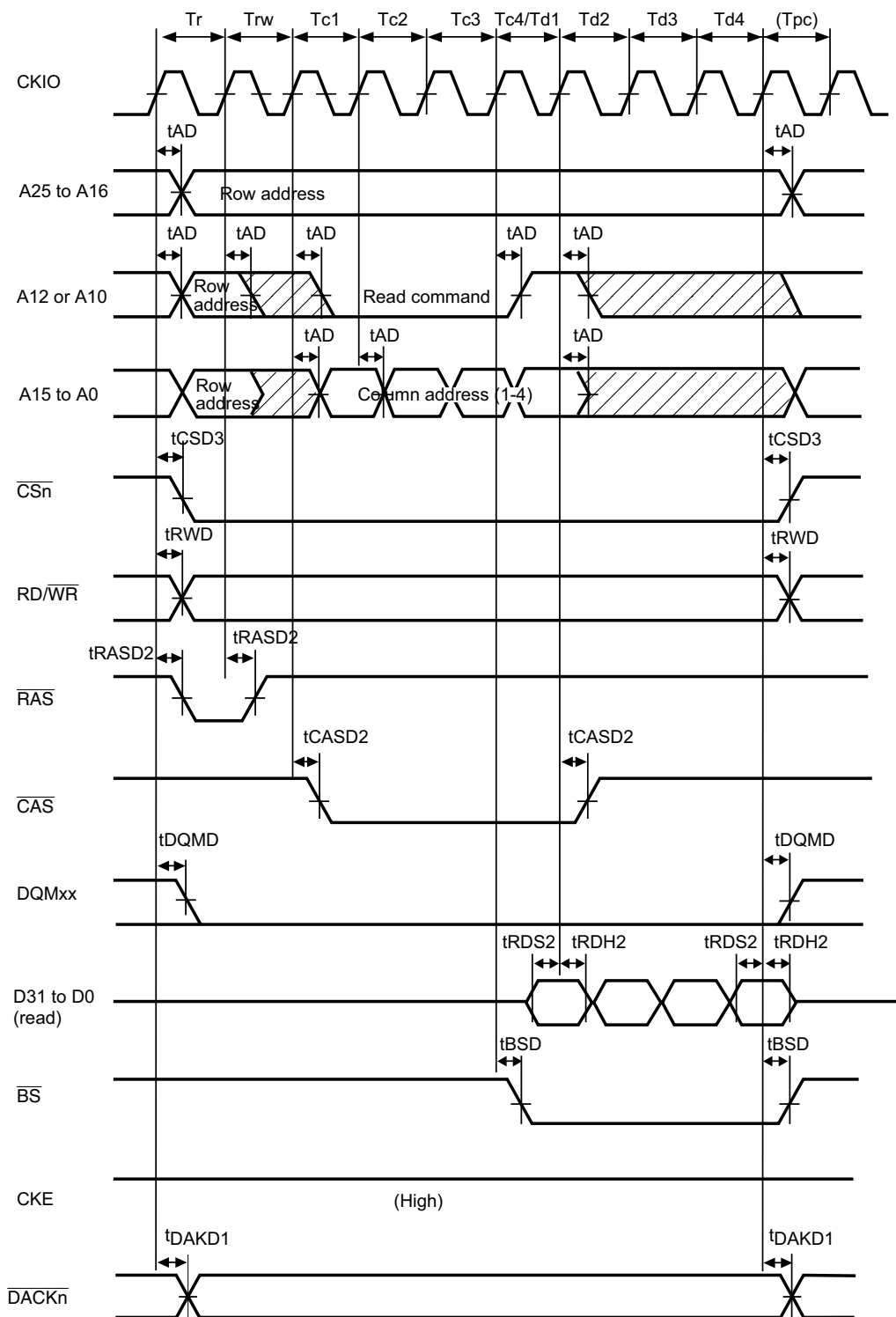
Figure 23.25 Synchronous DRAM Read Bus Cycle (Burst Read (Single Read x 4), RCD = 1, CAS Latency = 3, TPC = 0)
