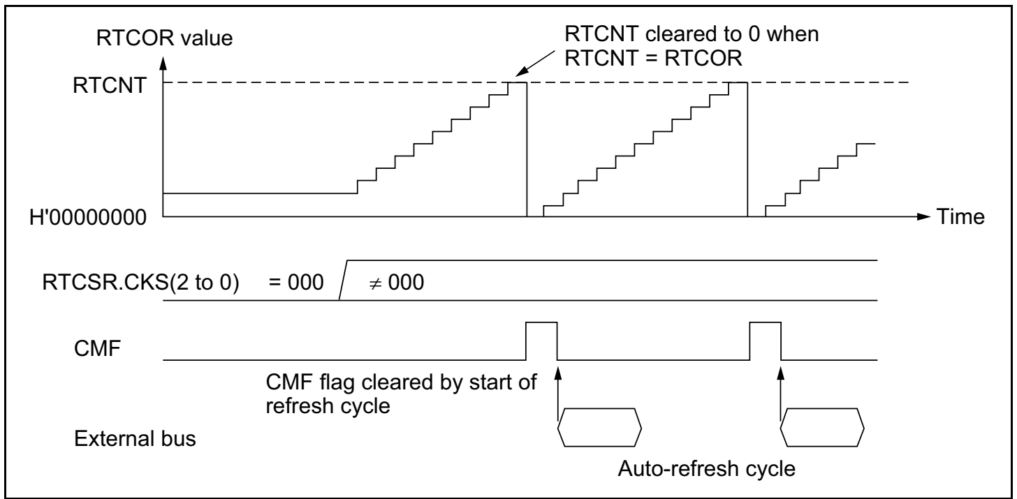
Figure 10.25 Auto-Refresh Operation
