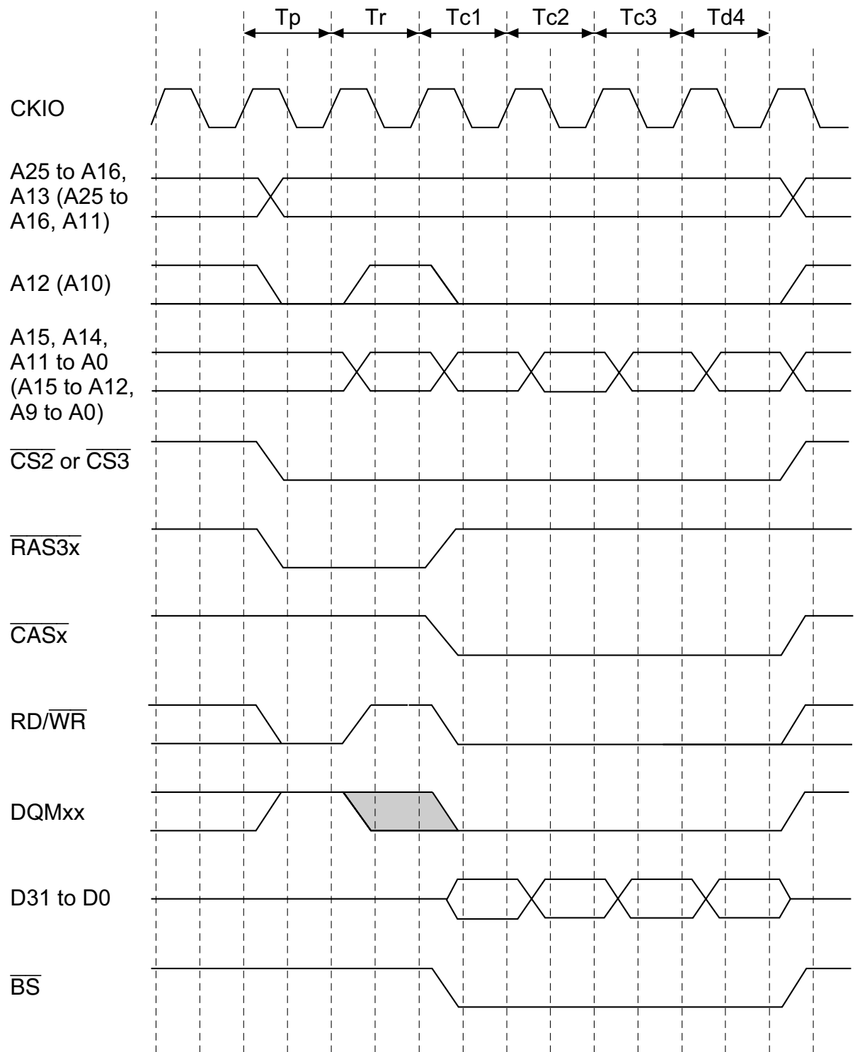
Figure 10.24 Burst Write Timing (Different Row Addresses)
