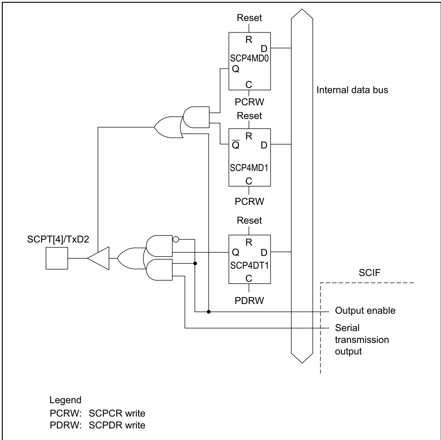
Figure 16.3 SCPT[4]/TxD2 Pin
