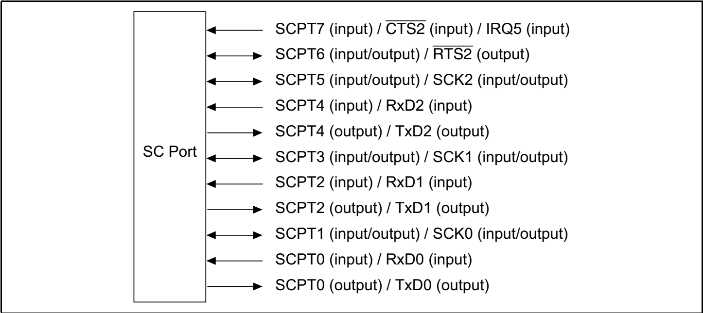
Figure 19.12 SC Port
