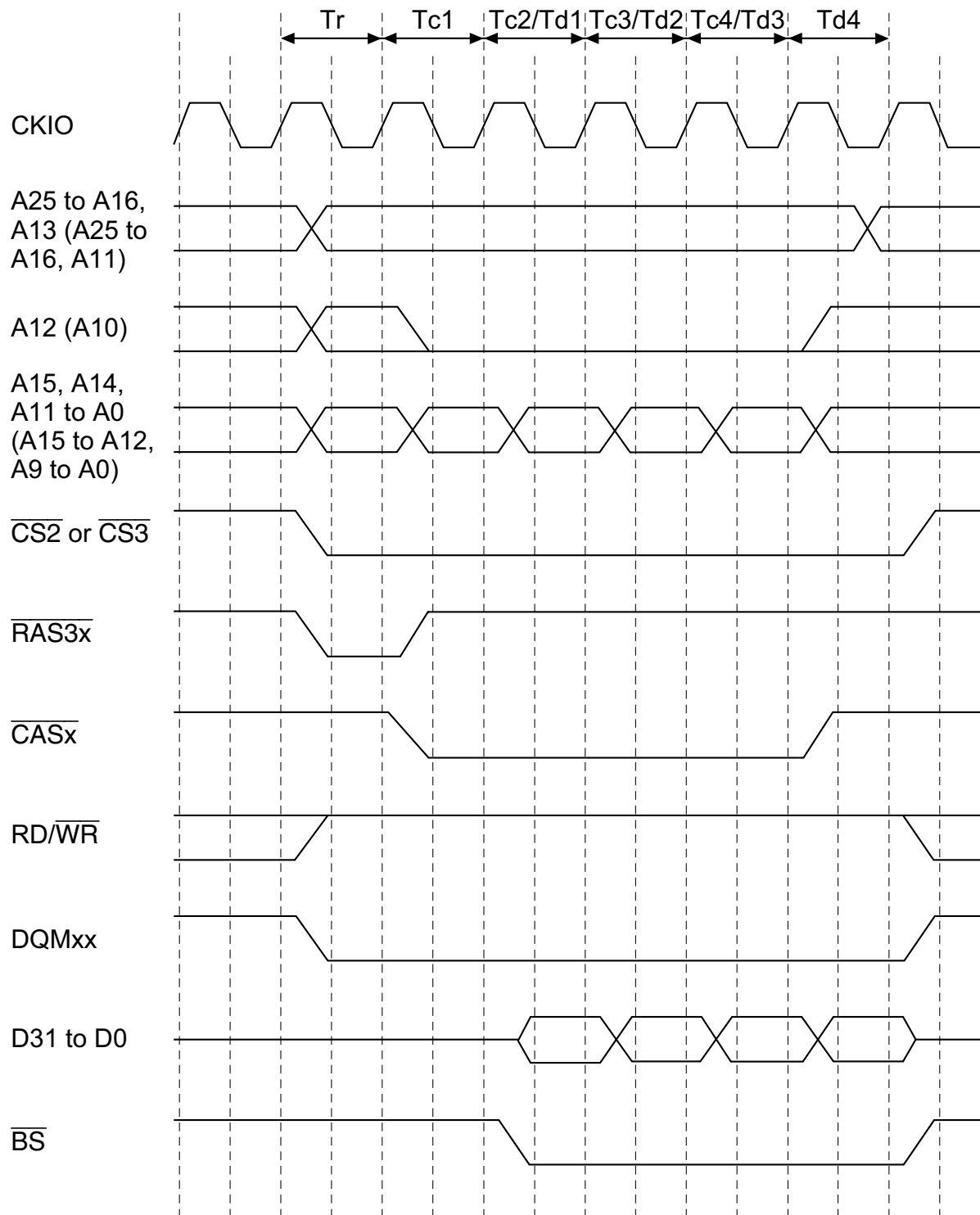
Figure 10.19 Burst Read Timing (No Precharge)
