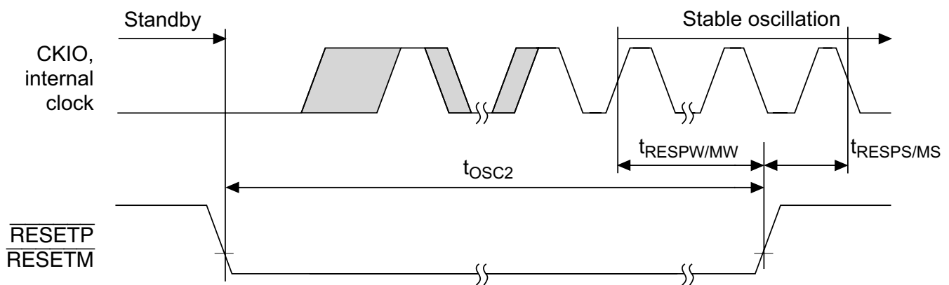
Figure 23.4 Power-on Oscillation Settling Time
