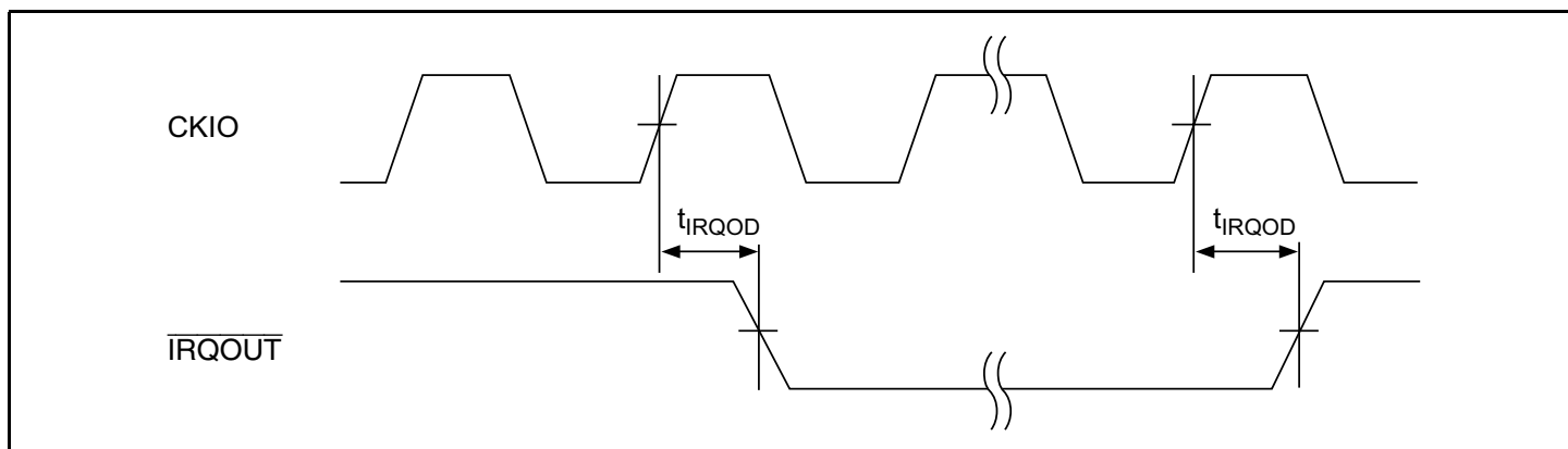
Figure 23.13 \overline{\text{IRQOUT}} Timing
