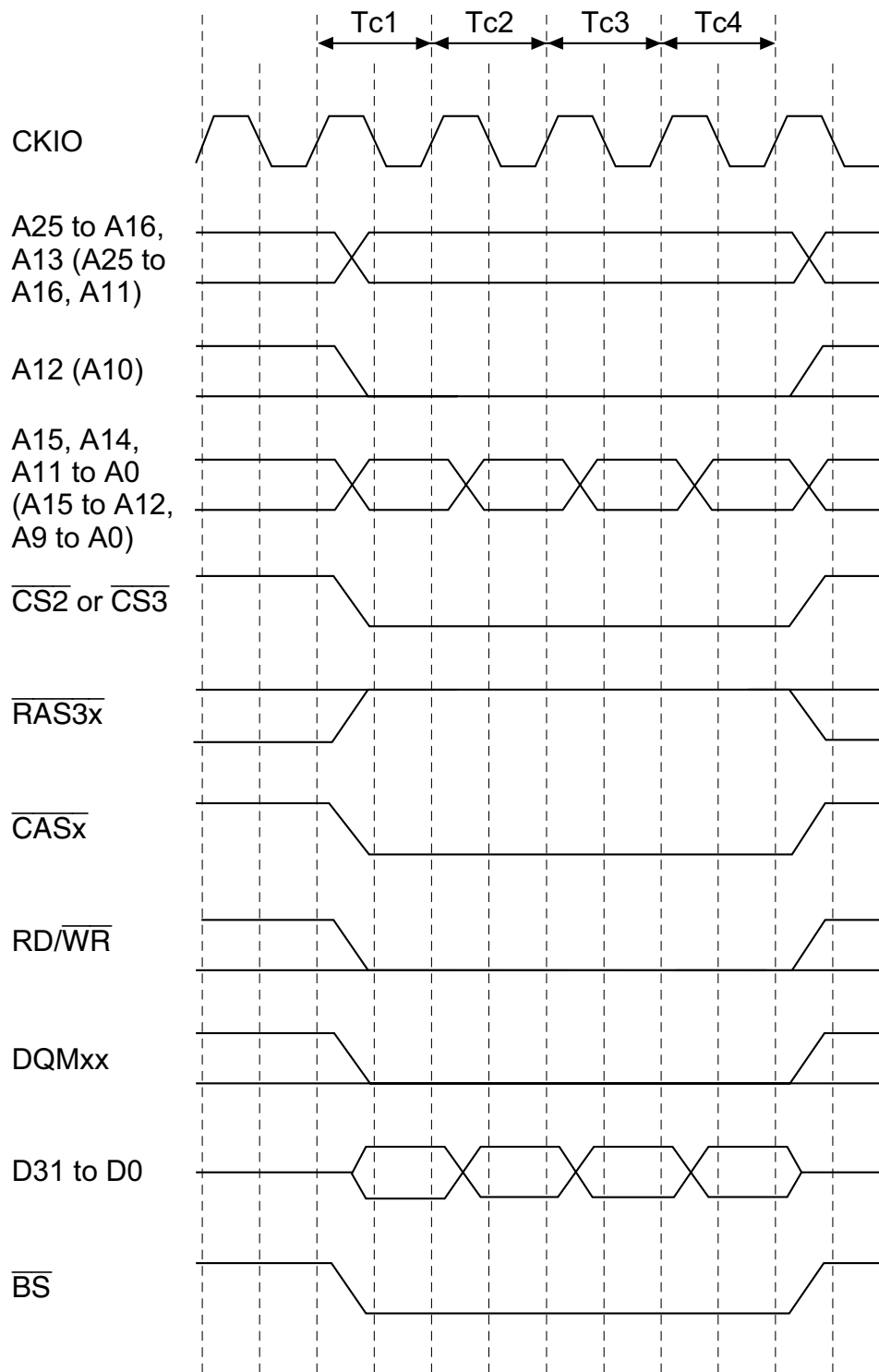
Figure 10.23 Burst Write Timing (Same Row Address)
