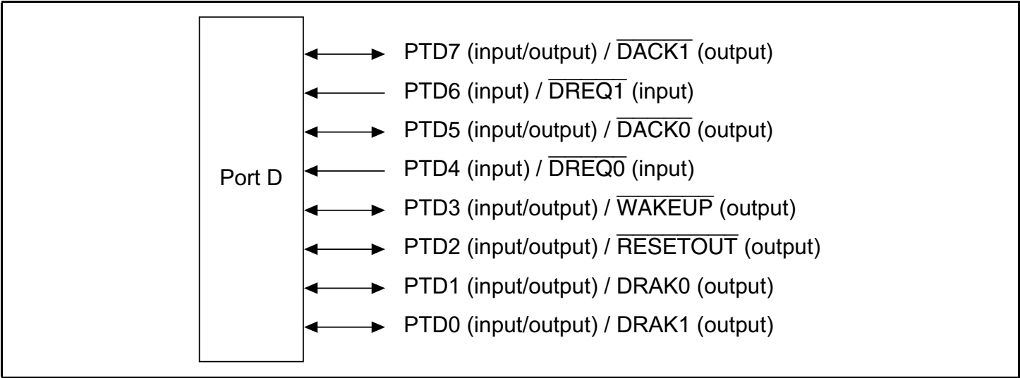
Figure 19.4 Port D
