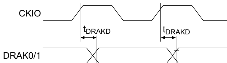
Figure 23.54 DRAK Output Timing
