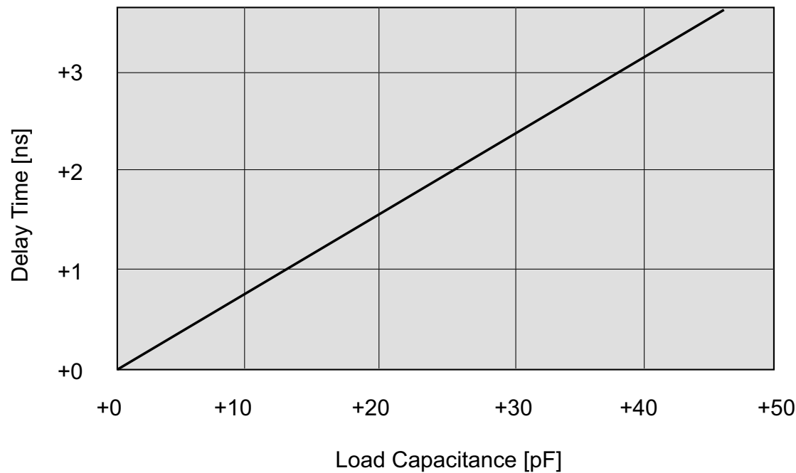
Figure 23.60 Load Capacitance vs. Delay Time
