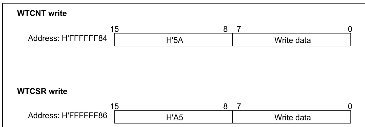
Figure 9.3 Writing to WTCNT and WTCSR
