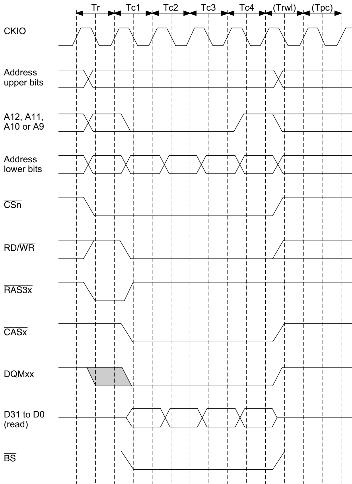
Figure 10.17 Basic Timing for Synchronous DRAM Burst Write
