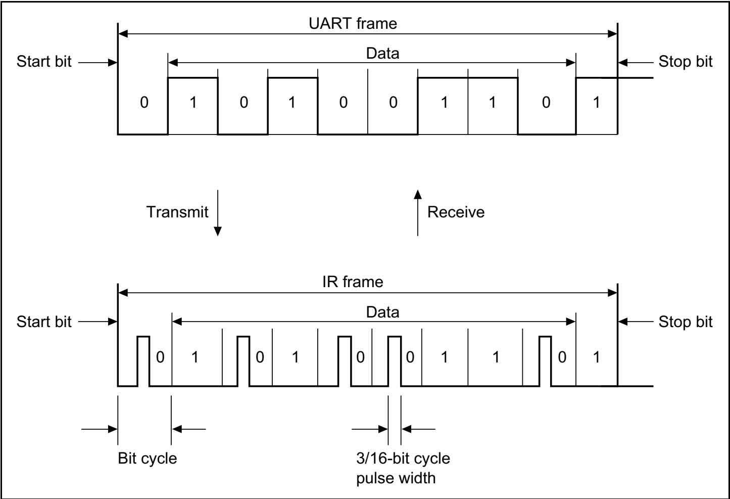
Figure 17.5 Transmit/Receive Operation
