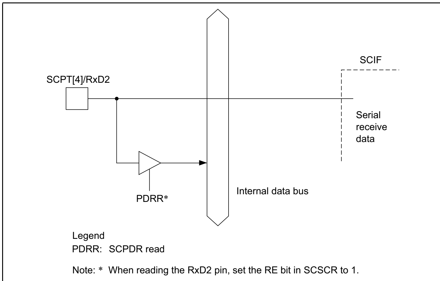
Figure 16.4 SCPT[4]/RxD2 Pin
