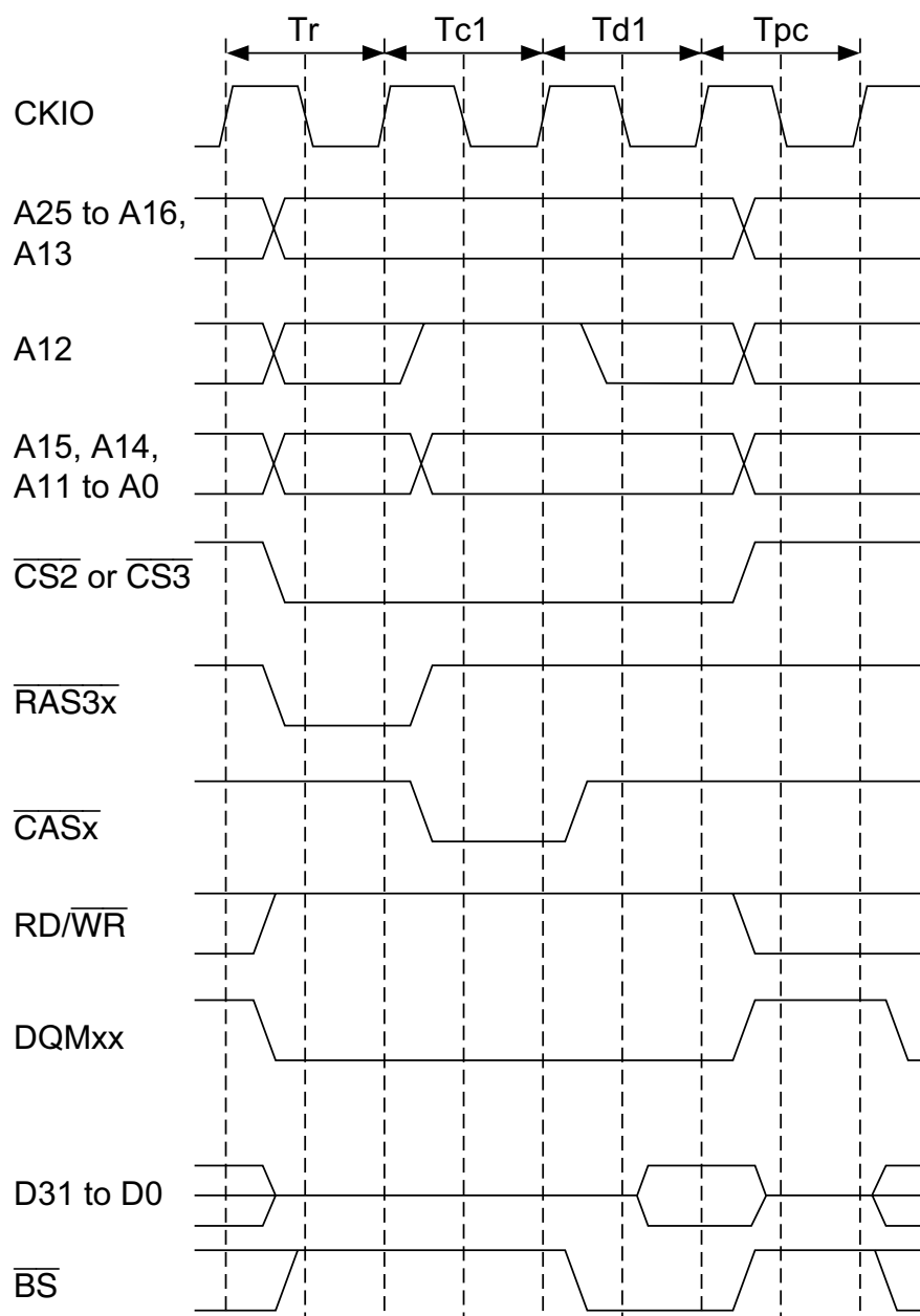
Figure 10.16 Basic Timing for Synchronous DRAM Single Read
