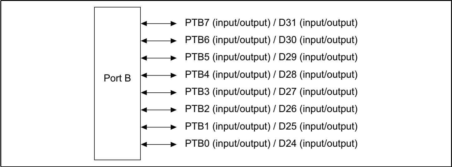
Figure 19.2 Port B
