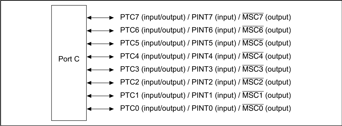
Figure 19.3 Port C
