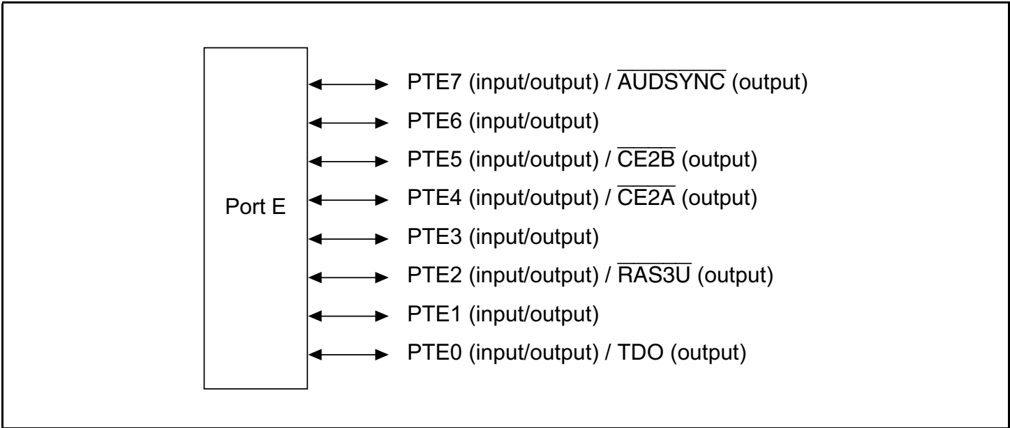
Figure 19.5 Port E
