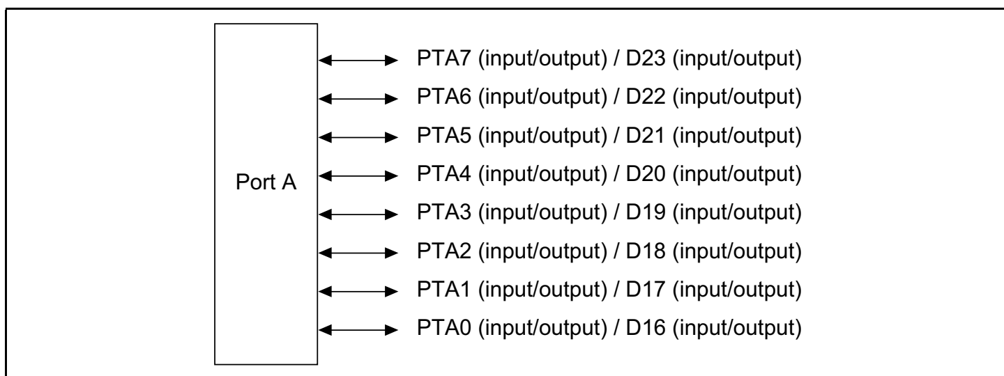
Figure 19.1 Port A
