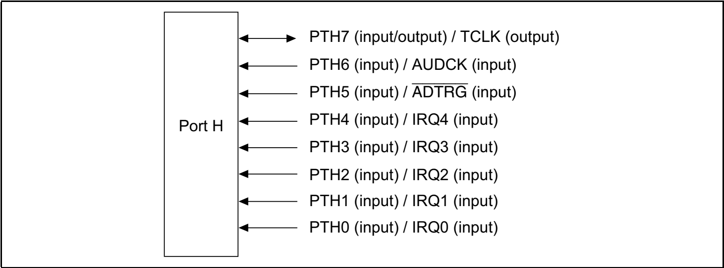
Figure 19.8 Port H
