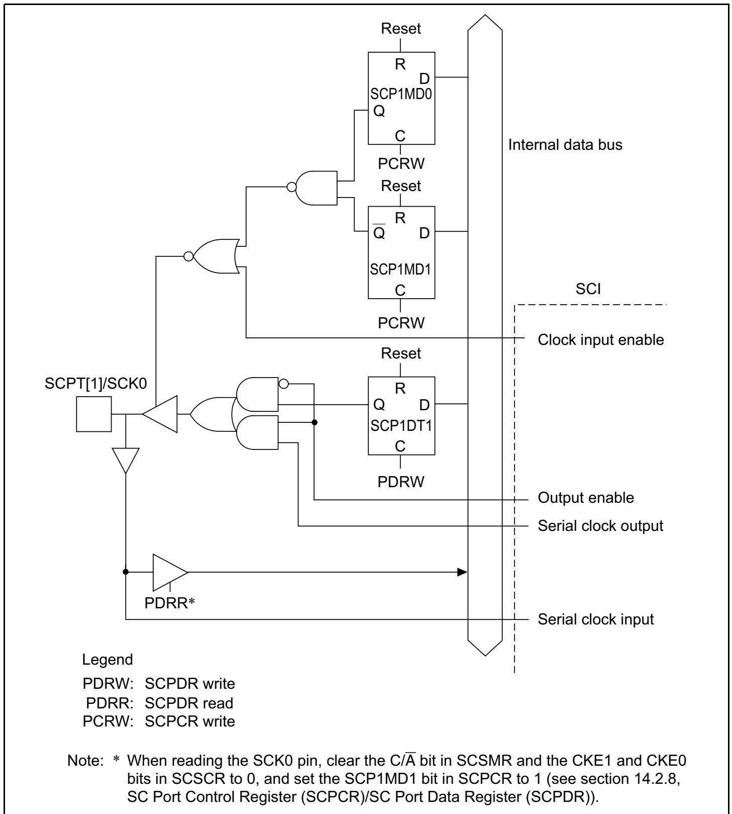
Figure 14.2 SCPT[1]/SCK0 Pin
