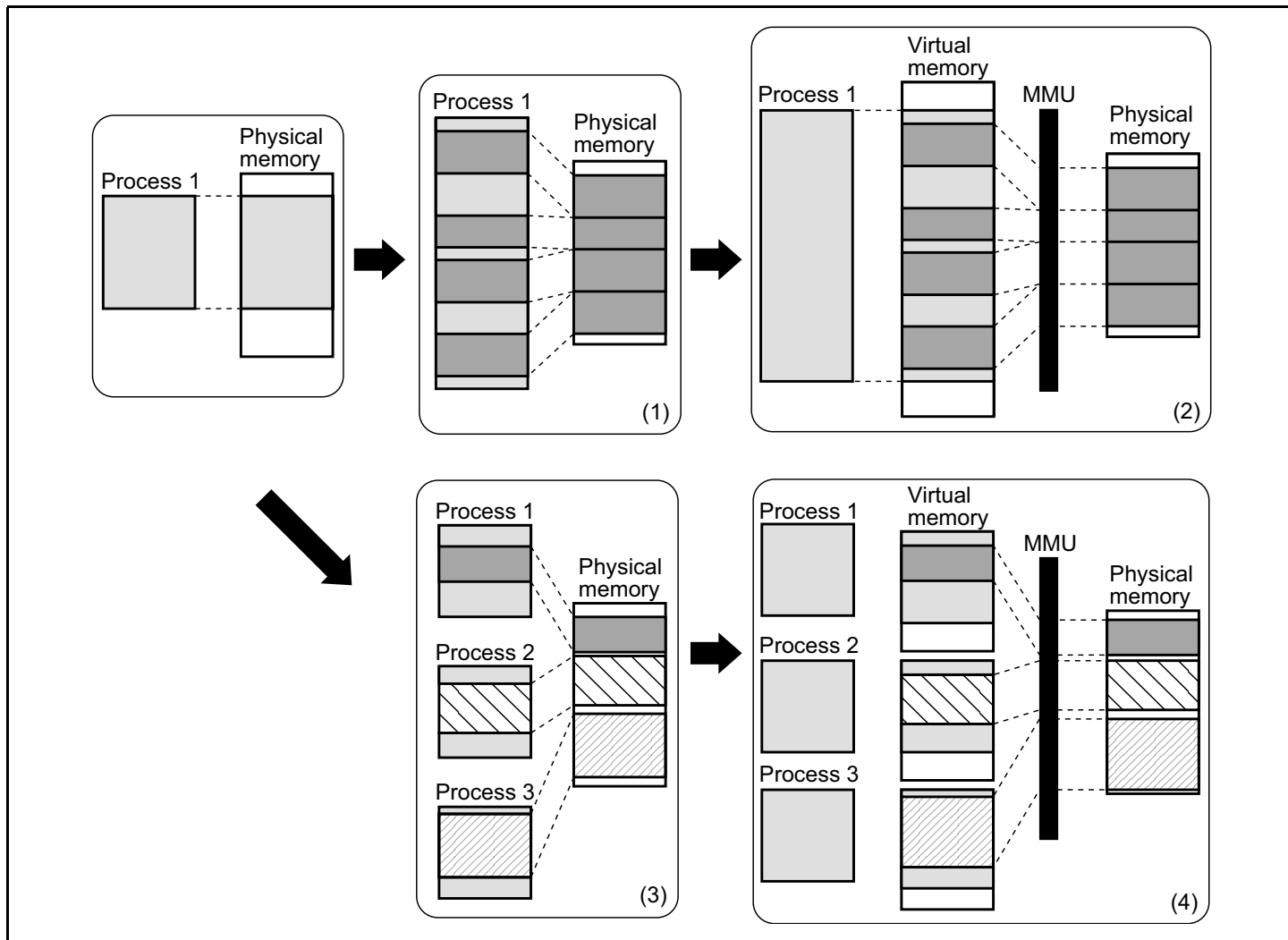
Figure 3.1 MMU Functions
