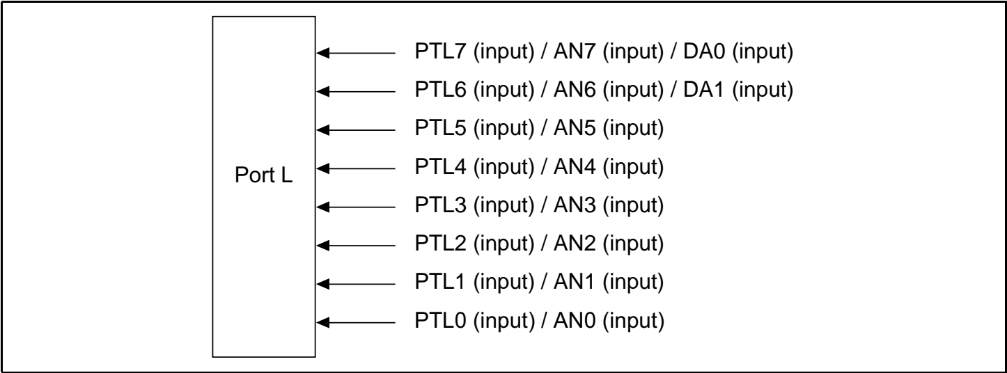
Figure 19.11 Port L
