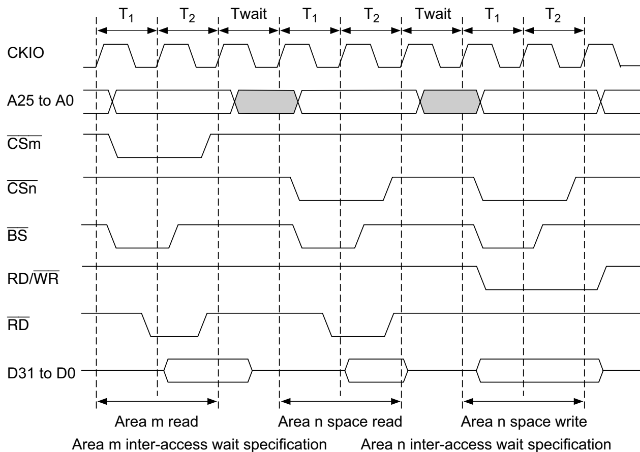
Figure 10.40 Waits between Access Cycles
