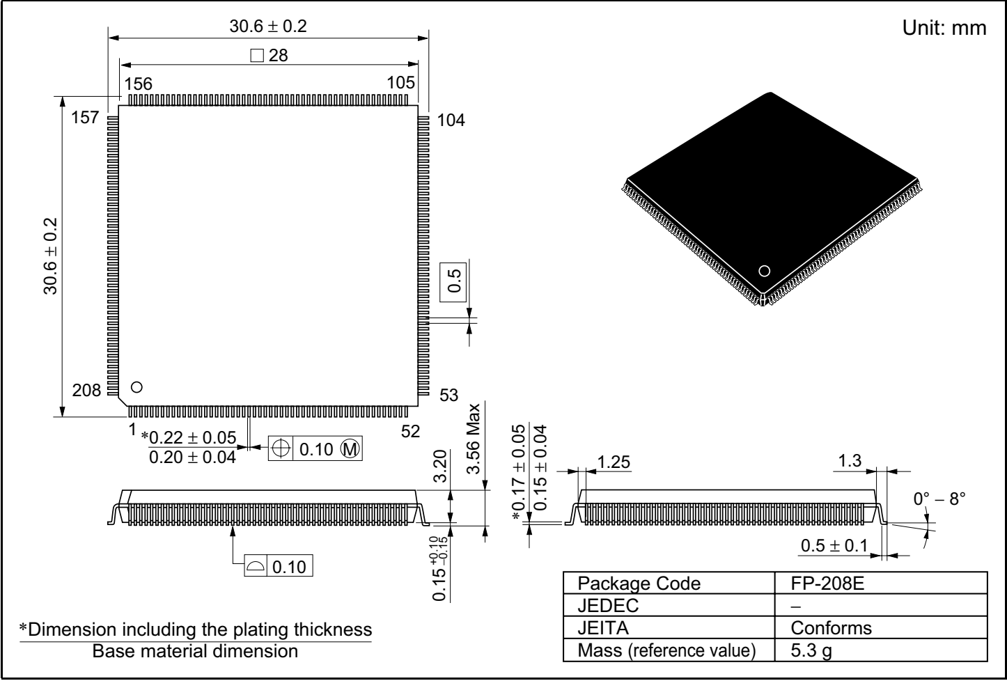
Figure D.2 Package Dimensions (FP-208E)
