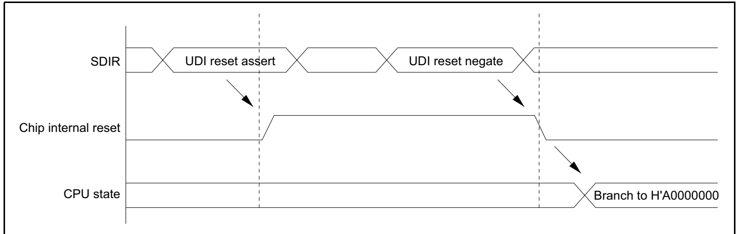
Figure 22.3 UDI Reset
