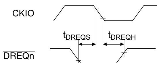
Figure 23.53 \overline{DREQ} Input Timing
