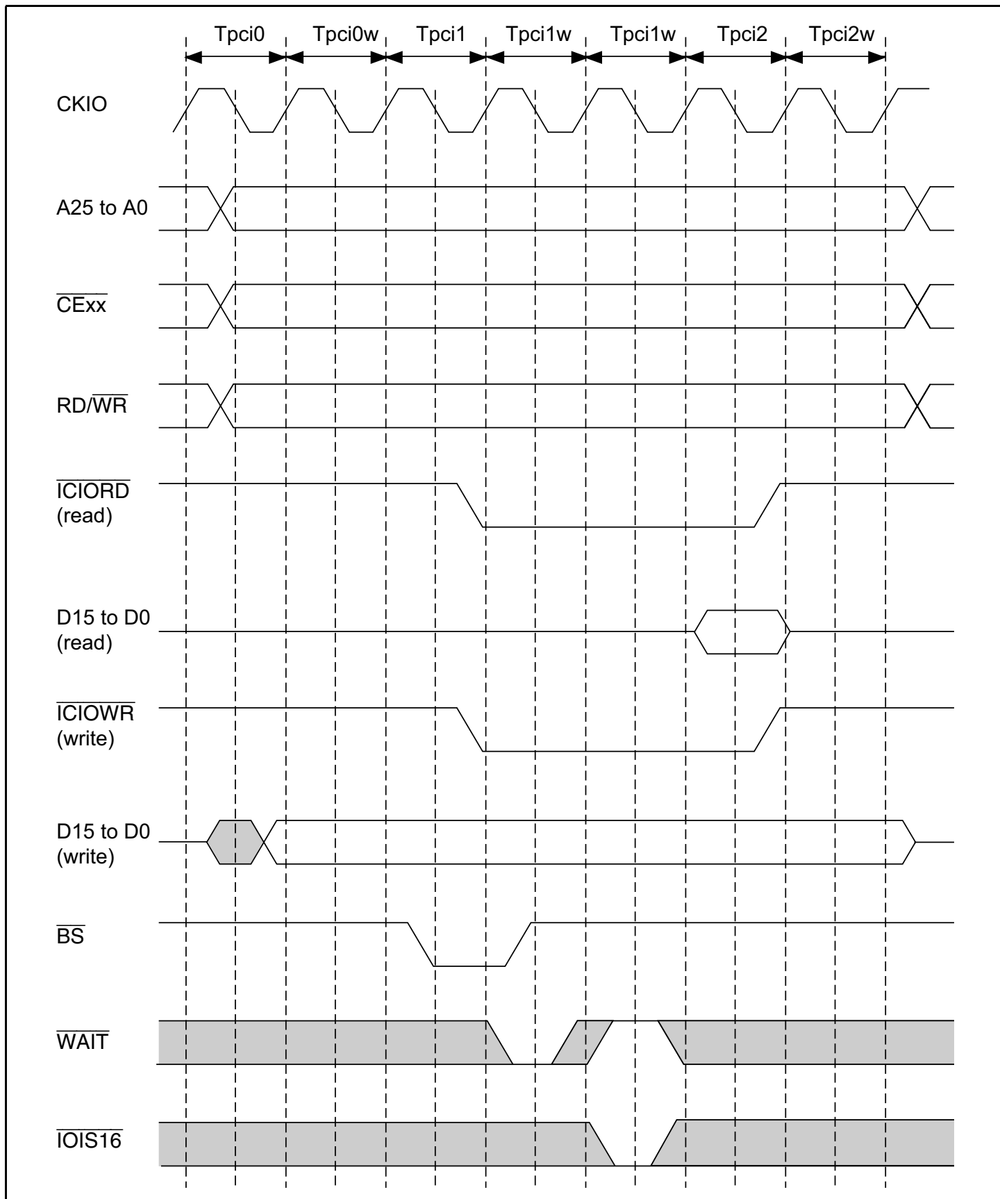
Figure 10.38 Wait Timing for PCMCIA I/O Card Interface
