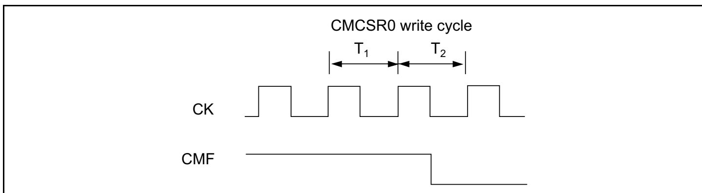
Figure 11.28 Timing of CMF Clearing by the CPU
