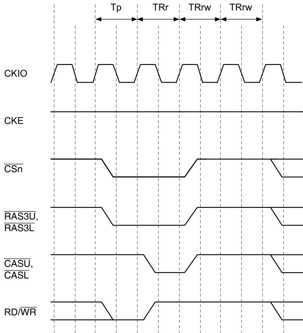
Figure 10.26 Synchronous DRAM Auto-Refresh Timing
