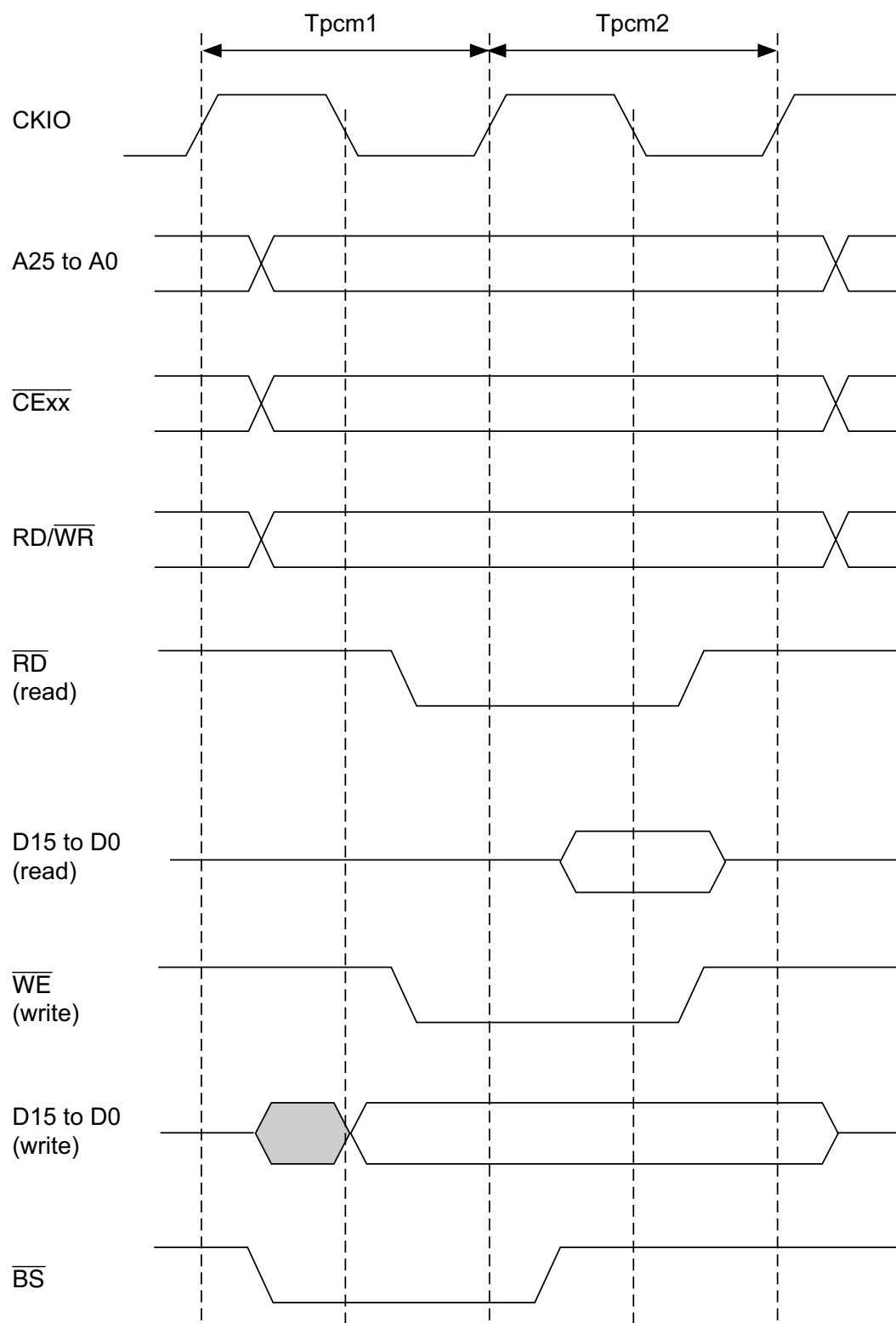
Figure 10.32 Basic Timing for PCMCIA Memory Card Interface
