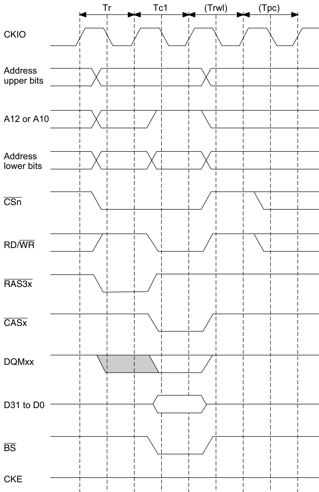
Figure 10.18 Basic Timing for Synchronous DRAM Single Write
