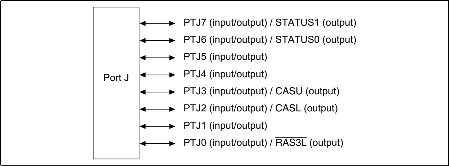
Figure 19.9 Port J
