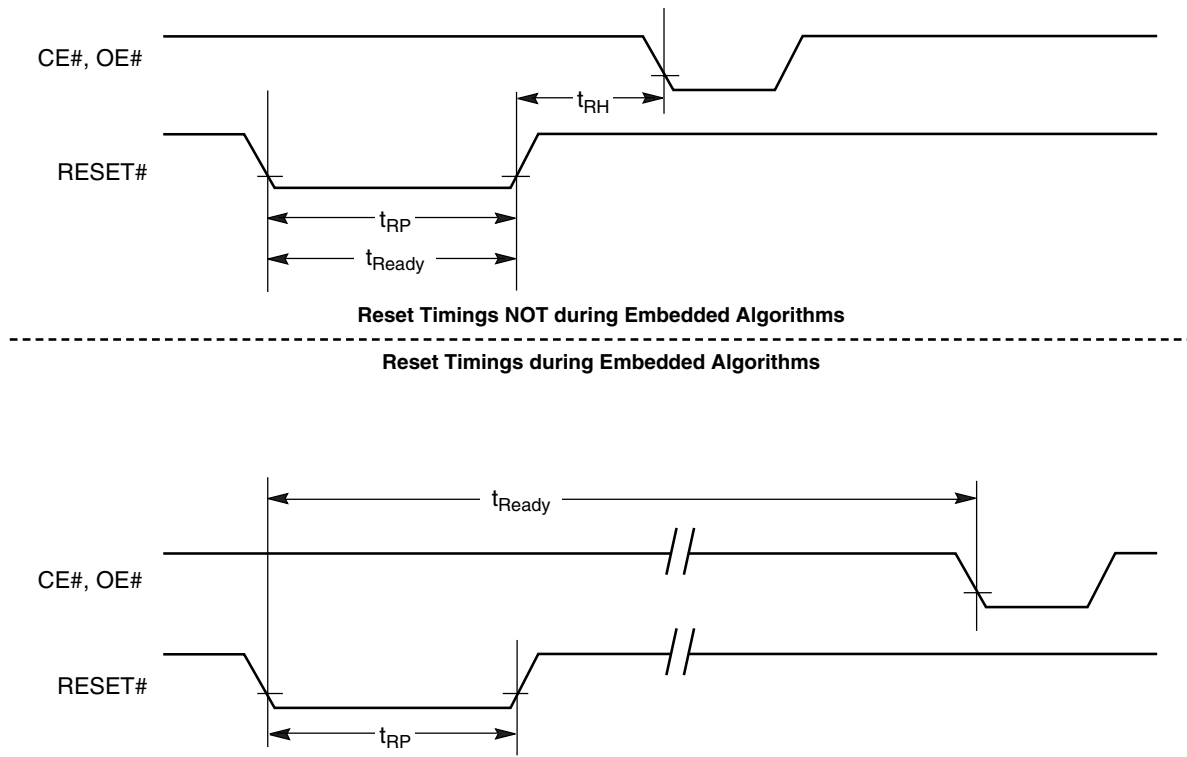
Figure 17. Reset Timings
