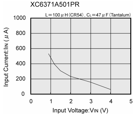
(4) No Load Input Current vs. Input Voltage
