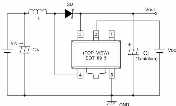
Circuit 3: XC6372E series
