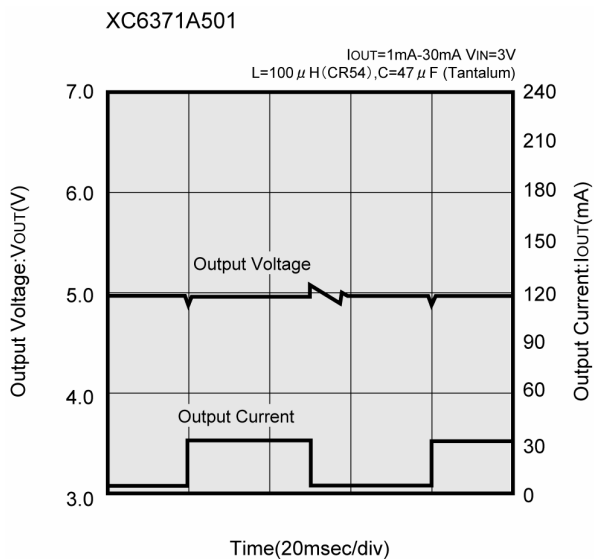
(6) Load Transient Response
