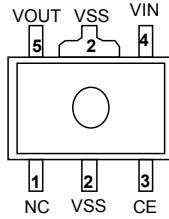
SOT-89-5 (TOP VIEW)
