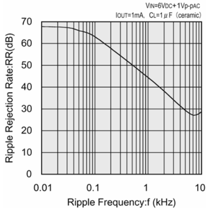
XC6202P502 (5.0V)
