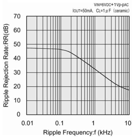
XC6202P502 (5.0V)
