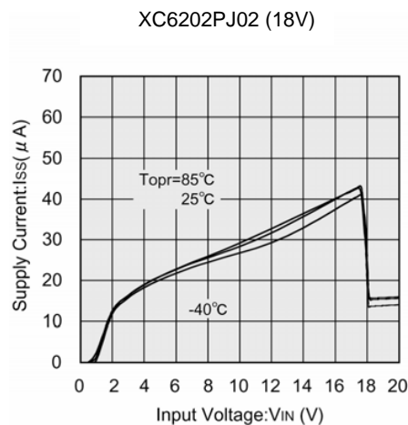
(4) Supply Current vs. Input Voltage
