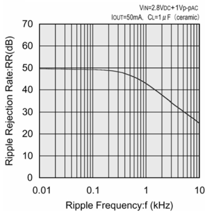
XC6202P182 (1.8V)
