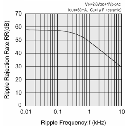
XC6202P182 (1.8V)
