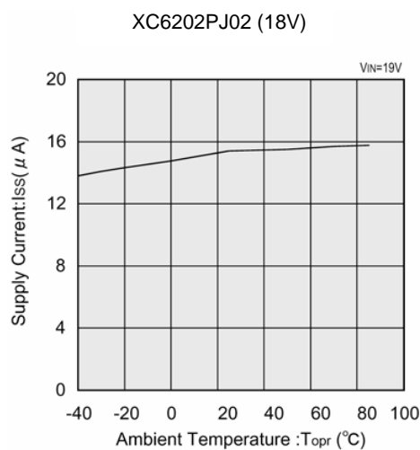
(6) Supply Current vs. Ambient Temperature
