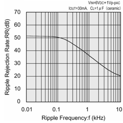
XC6202P502 (5.0V)
