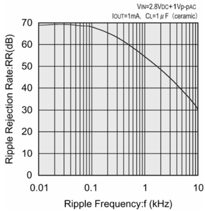
XC6202P182 (1.8V)
