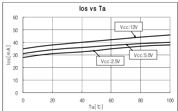
Fig.6 Output Short circuit current vs Ambient Temperature
