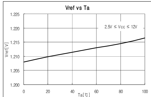
Fig.2 Vref vs Ambient Temperature
