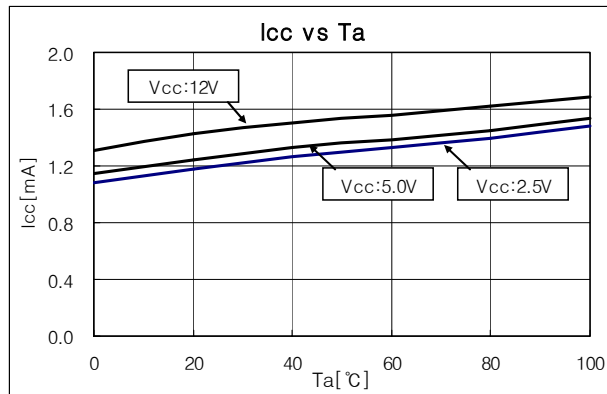
Fig.1 Supply current vs Ambient Temperature
