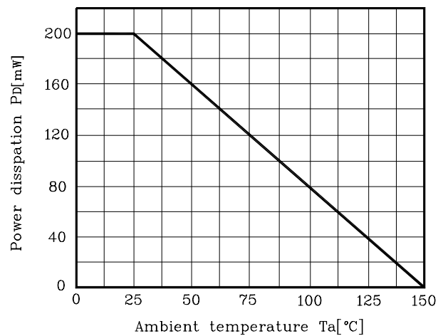
Fig. 1 P_D - T_a
