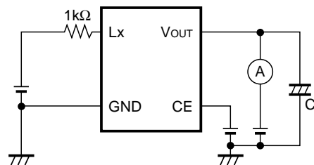
Test Circuit 2
