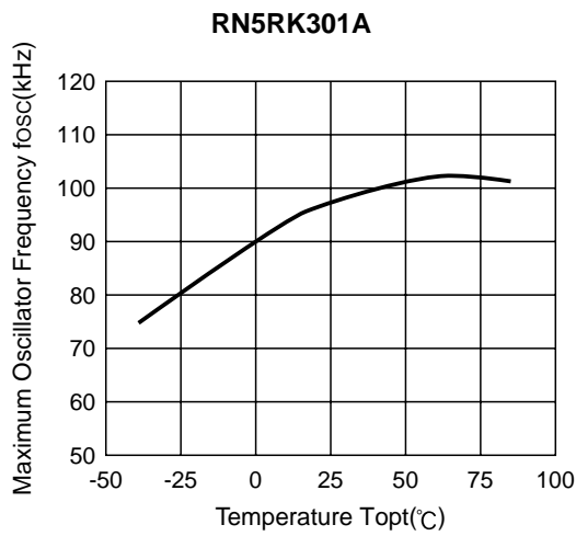
15) Maximum Oscillator Frequency vs. Temperature
