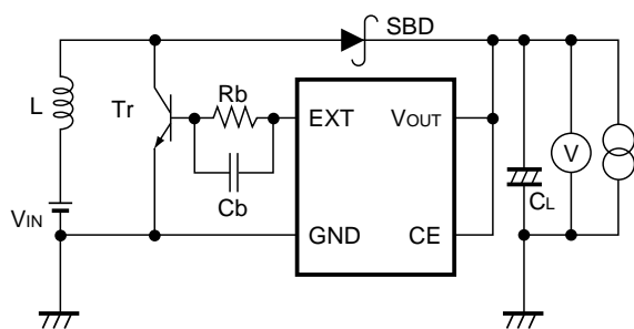
Test Circuit 1
