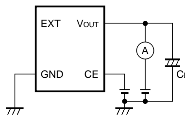
Test Circuit 2
