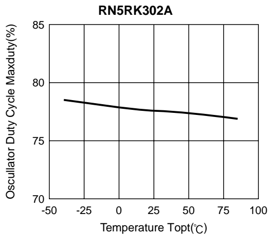
11) Oscillator Duty Cycle vs. Temperature
