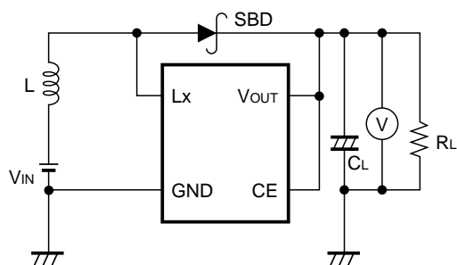
Test Circuit 1
