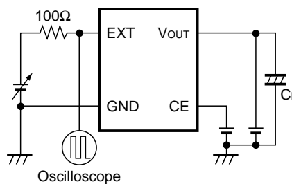
Test Circuit 4
