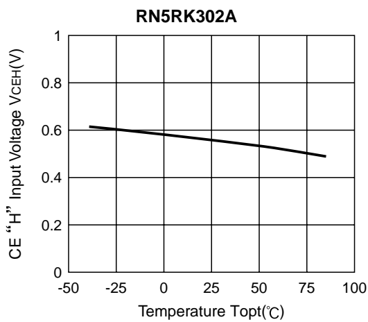
13) CE "H" Input Voltage vs. Temperature
