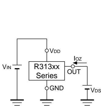
Test Circuit for Off Leakage Current
