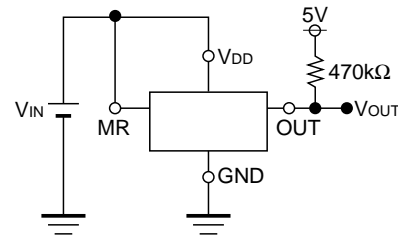
Test Circuit for Detector Threshold (CMOS Output type; pull-up part is not necessary.)
