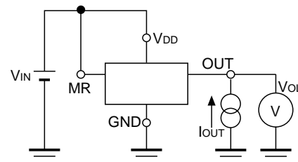
Test Circuit for "L" Output Voltage
