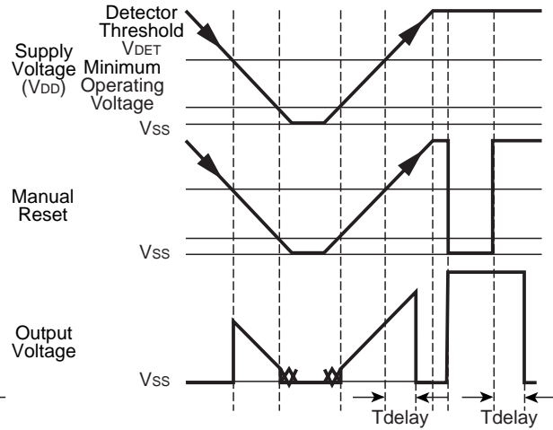
R3133x Operation Diagram
