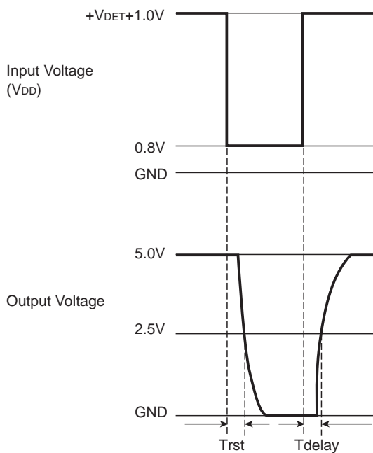
Nch Open Drain Output
