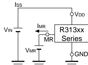
Test Circuit for MR pin Pull-up Resistance
