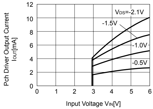
R3130N29xx3
