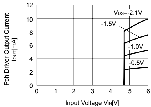
R3130N46xx5
