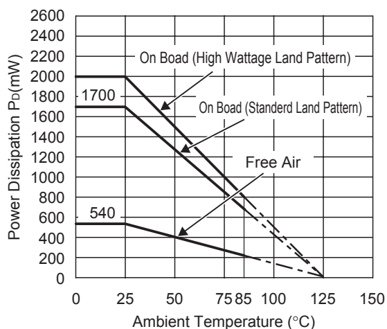
Power Dissipation
