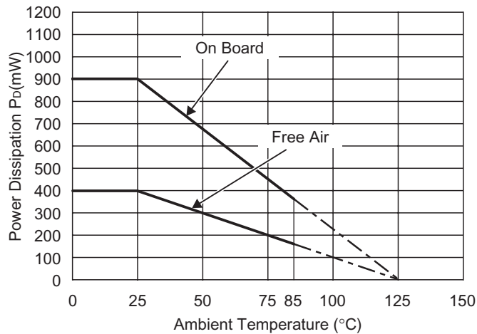
Power Dissipation
