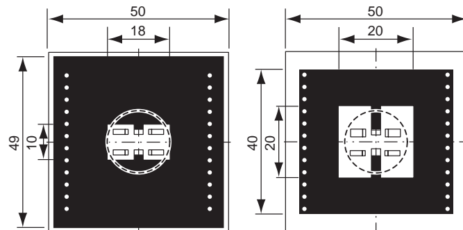
High Wattage Standard Measurement Board Pattern
