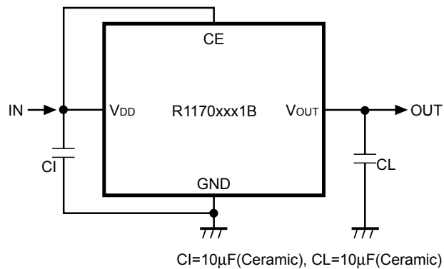
Example of the typical application of R1170xxxxB
