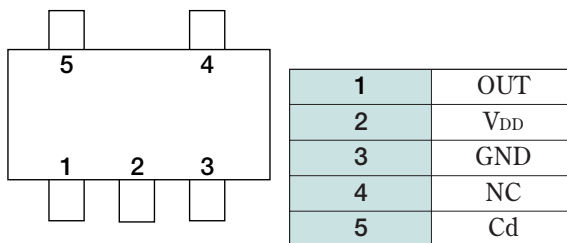
SOT-25A (TOP VIEW)
