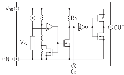
■ PST35XXUR (SC-82ABA/-82ABB)
