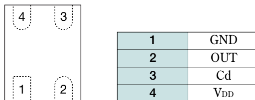
SSON-4A (TOP VIEW)
