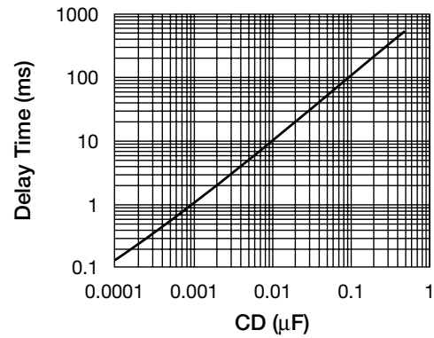
■ Delay time vs CD
