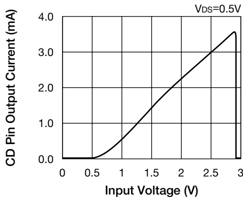
■ CD pin output current vs input voltage
