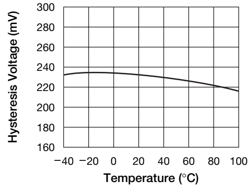
■ Hysteresis voltage vs temperature
