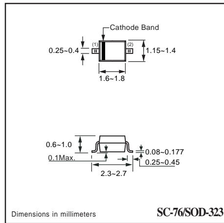
SC-76/SOD-323
