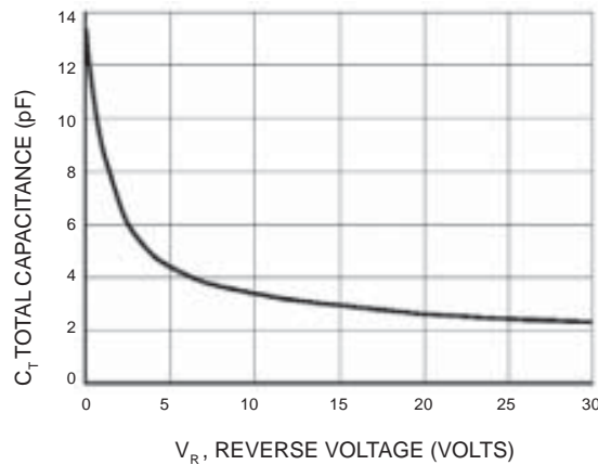
Figure 4. Total Capacitance
