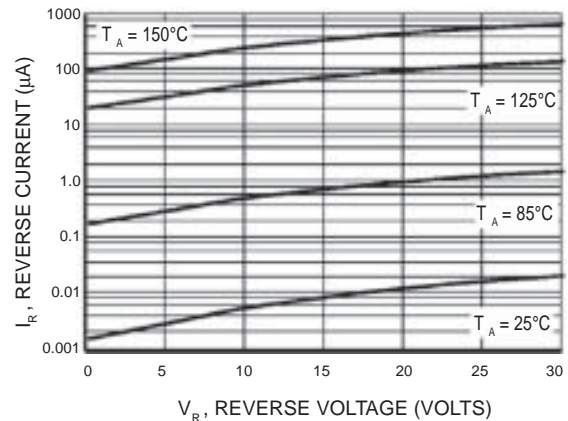
Figure 3. Leakage Current
