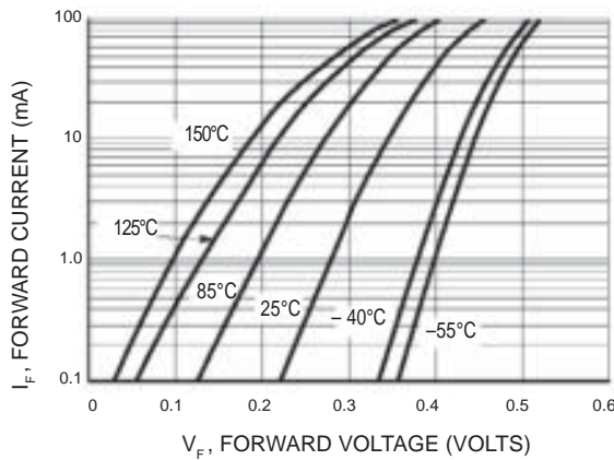
Figure 2. Forward Voltage
