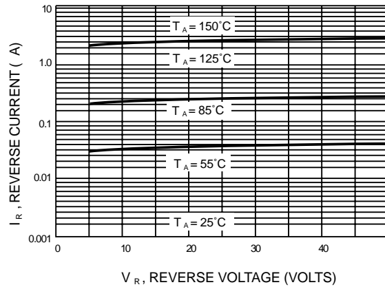
Figure 3. Leakage Current
