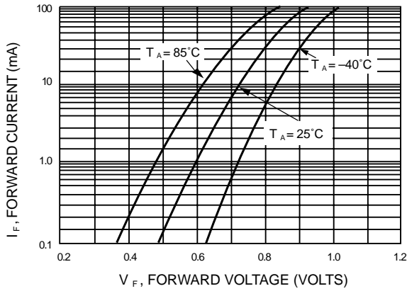
Figure 2. Forward Voltage
