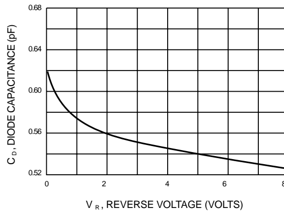
Figure 4. Capacitance
