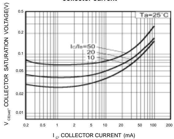
Fig.6 Collector-emitter saturation voltage vs. collector current
