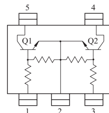
EQUIVALENT CIRCUIT (TOP VIEW)
