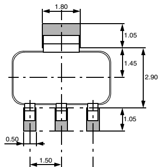
Fig. 3–6: Recommended pad size SOT89B-1 Dimensions in mm
