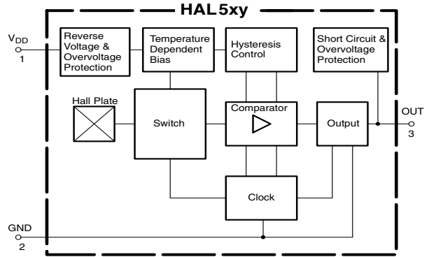
Fig. 2-1: HAL 5xx block diagram
