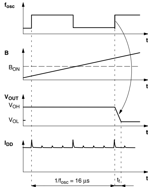
Fig. 2-2: Timing diagram
