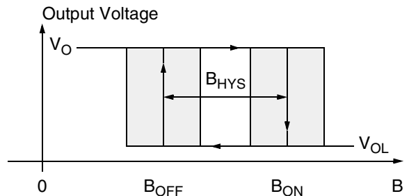
Fig. 4–45: Definition of magnetic switching points for the HAL 523
