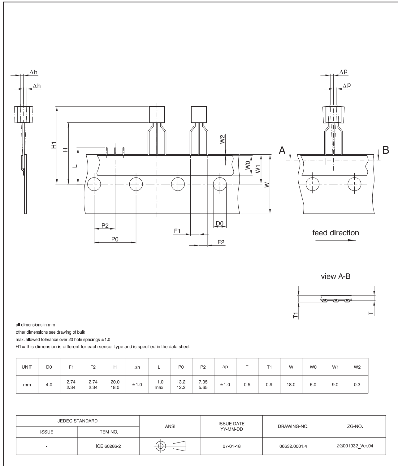
Fig. 3-4: T092UA-1: Dimensions ammpack inline, spread
