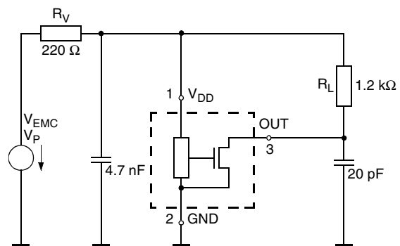
Fig. 5–1: Test circuit for EMC investigations
