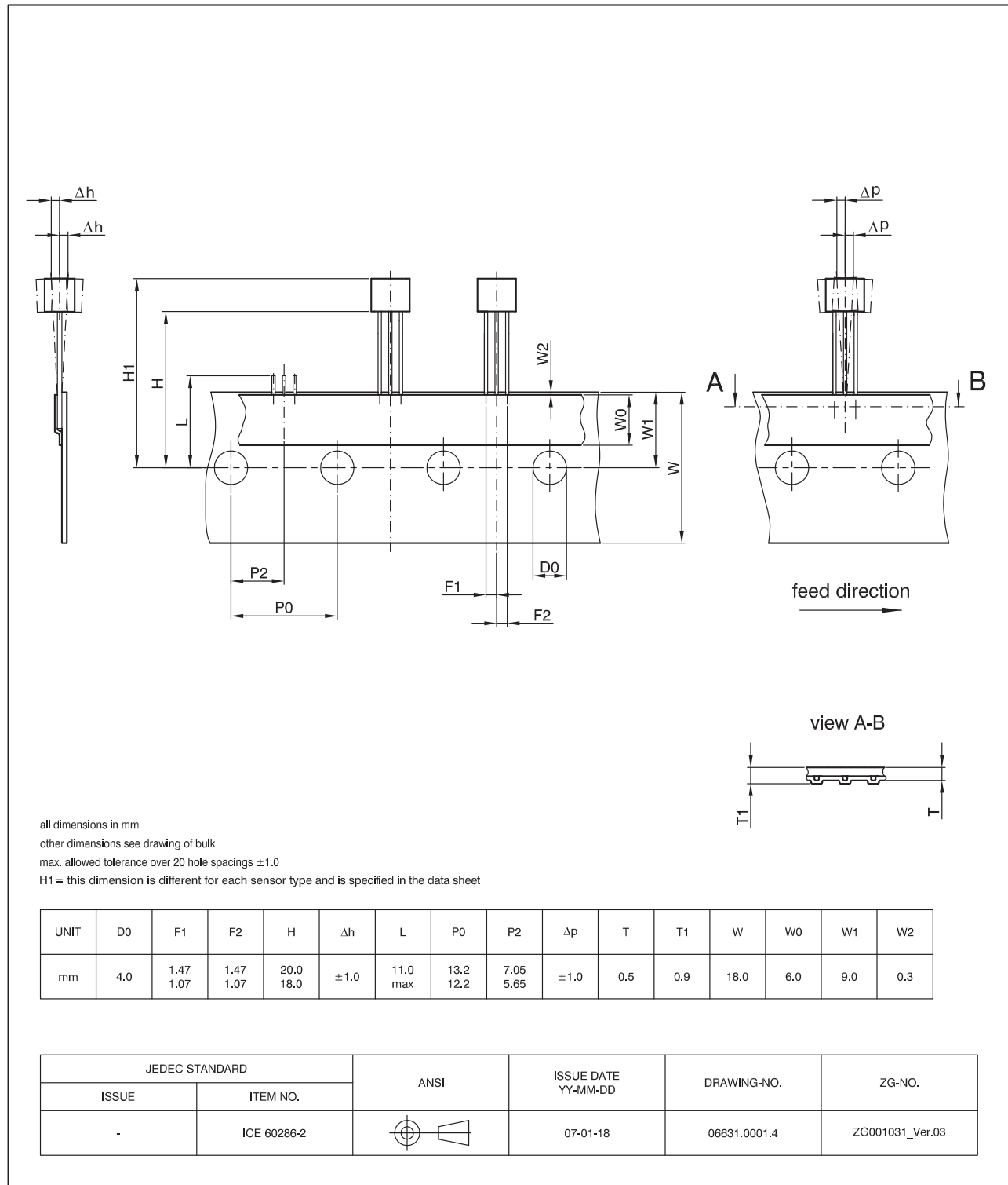
Fig. 3-5: TO92UA-2: Dimensions ammopack inline, not spread
