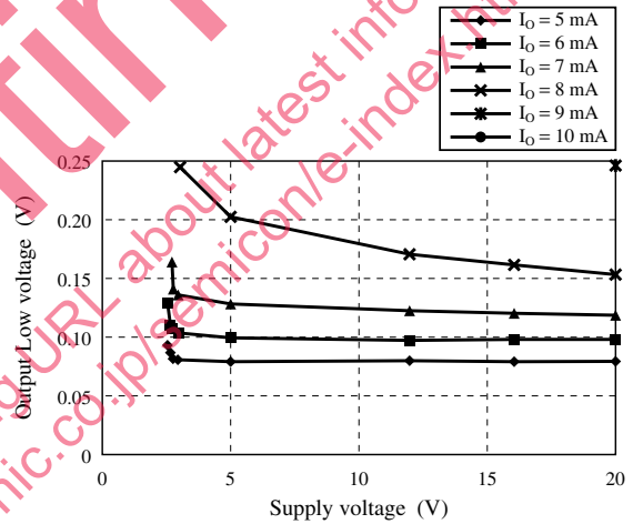
Output low voltage — Supply voltage (Temp. = 50°C)
