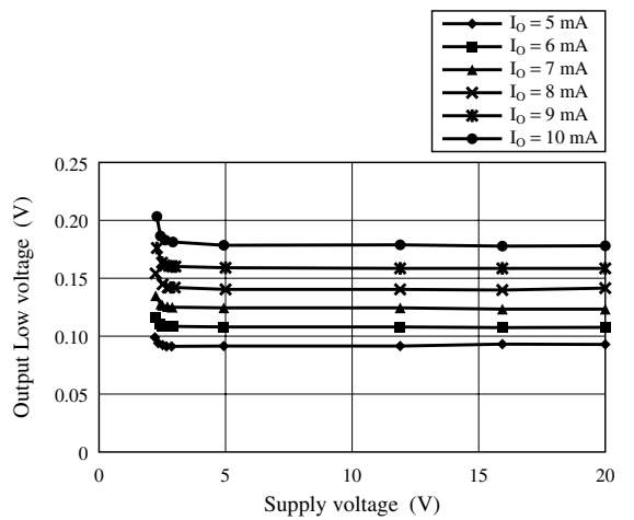
Output low voltage — Supply voltage (Temp. = 150°C)
