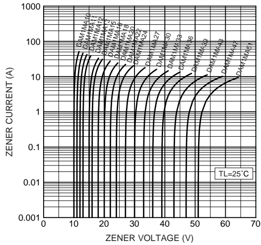
Typical zener characteristics ( Vz:10~51V)
