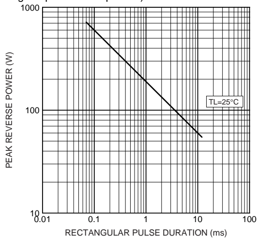
Typical reverse power characteristic (Rectangular pulse non-repetitive)
