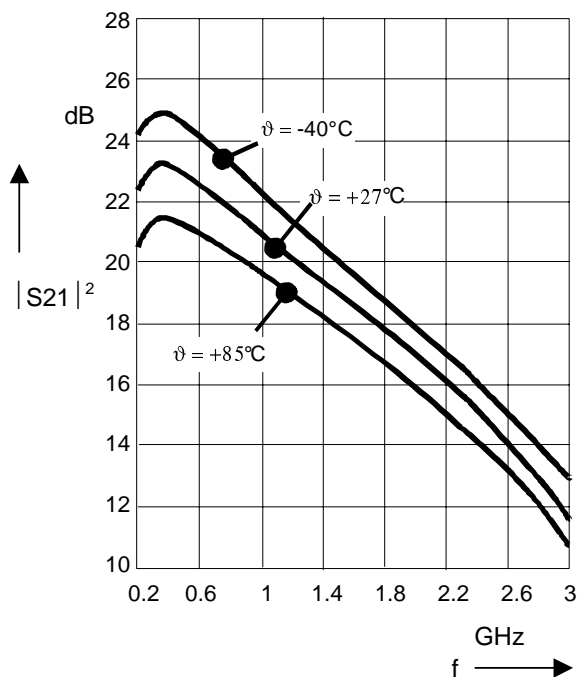
|S21|^2 versus Frequency and Temperature Vcc=3V, Icc=7mA
