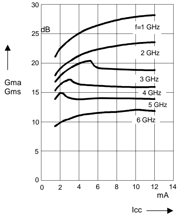
Power Gain versus Device Current Vcc=3V
