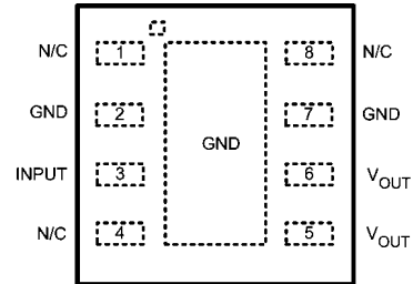
882246 Pin 2 and pin 7 are fused to center DAP Pin 5 and 6 need to be tied together on PCB board Top View See NS Package Number LDC08A
