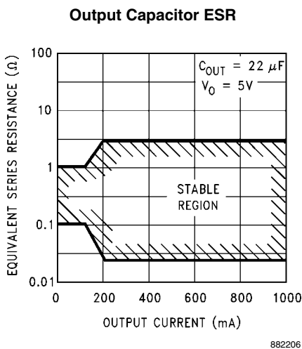
FIGURE 1. ESR Limits
