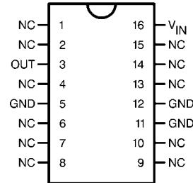
882244 Top View See NS Package Number WG16A
