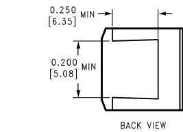
3-Lead TO-263 Surface Mount Package (MP) Order Number LM2940S-5.0, LM2940S-8.0, LM2940S-9.0, LM2940S-10, LM2940S-12, LM2940CS-5.0, LM2940CS-12 or LM2940CS-15 NS Package Number TS3B
