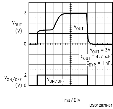
Turn-ON Waveform
