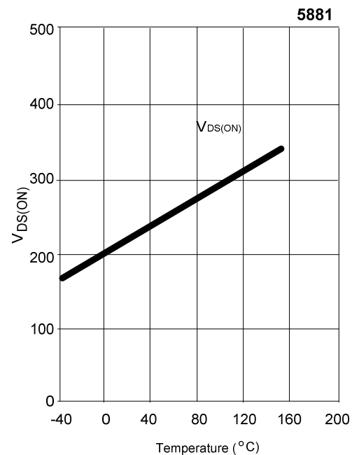
11.4 Typical Saturation Voltage vs Temperature ( V_{DD}=12V ; I_{out}=20mA )
