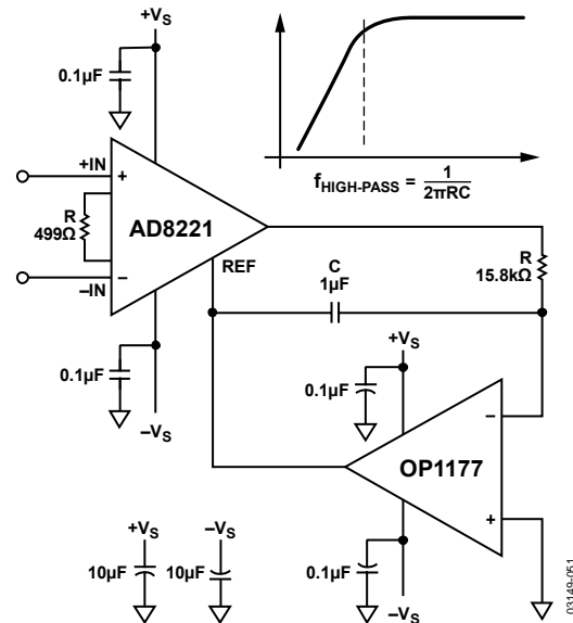
Figure 51. AC-Coupled Circuit
