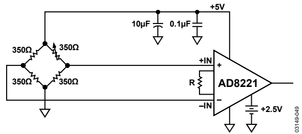
Figure 49. Precision Strain Gage
