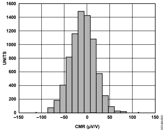
Figure 3. Typical Distribution for CMR (G = 1)
