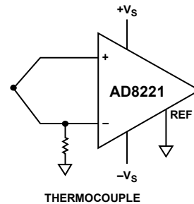
THERMOCOUPLE
