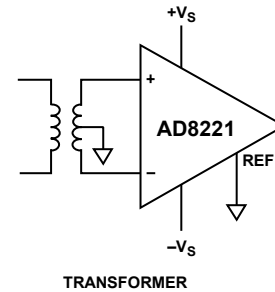
TRANSFORMER
