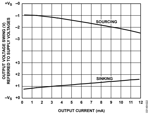
Figure 22. Output Voltage Swing vs. Output Current, G = 1
