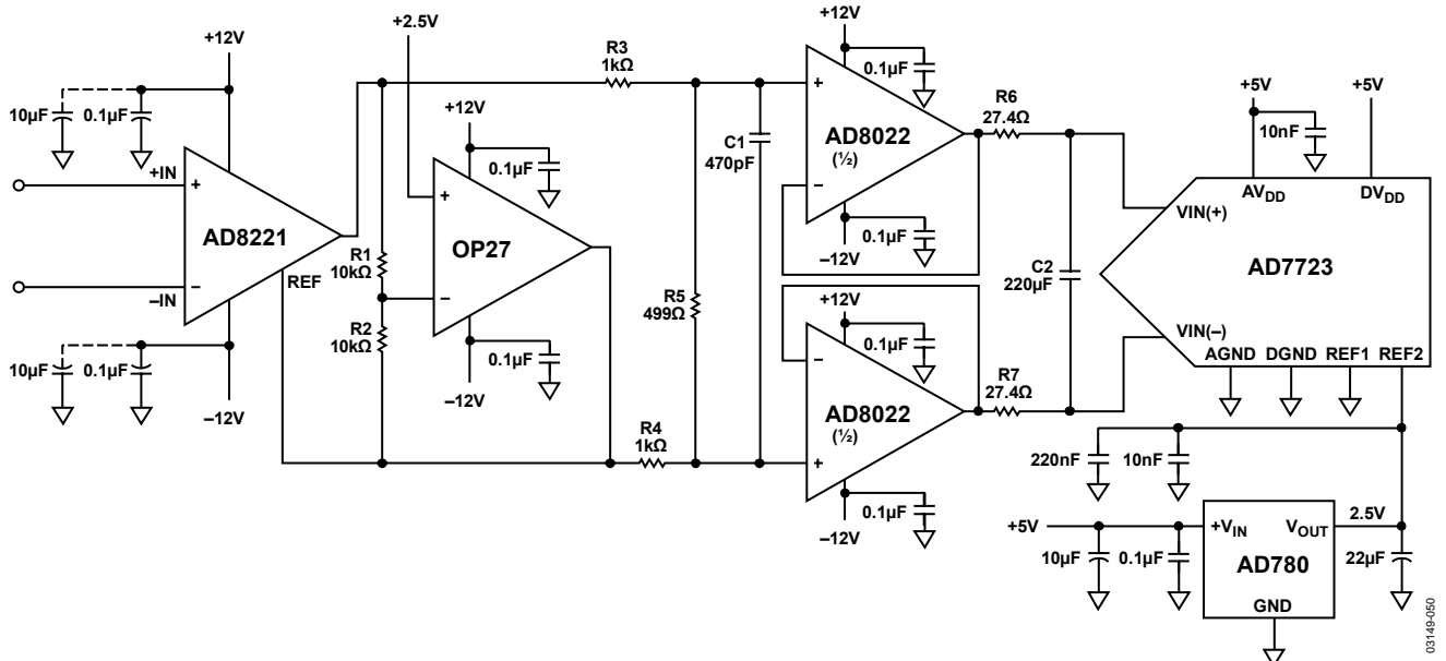
Figure 50. Interfacing to a Differential Input ADC
