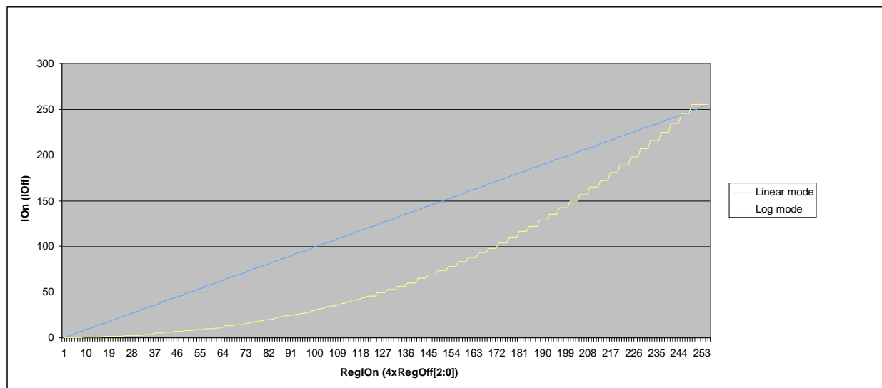
Figure 19 – LED Driver Linear vs Logarithmic Function (II)
