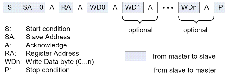
Figure 8 - 2-Wire Serial Interface, Write Operation
