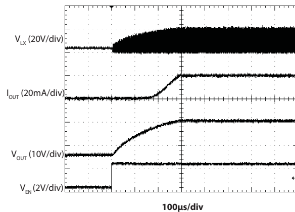
Start-Up Response
