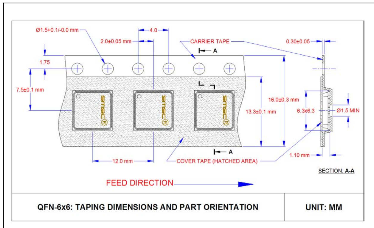
Figure 9.2 QFN, 6x6 Tape &amp; Reel
