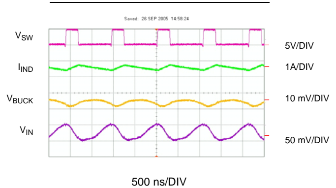
Figure 24: Switching Waveforms - PWM mode
