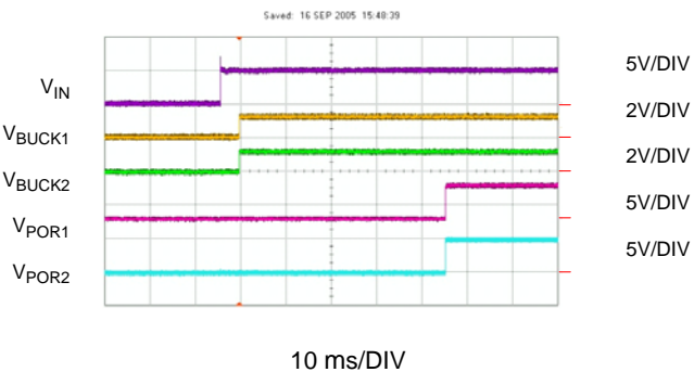
Figure 19: Hot Plug
