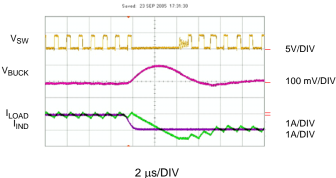
Figure 31: Slow Load Fall Time
