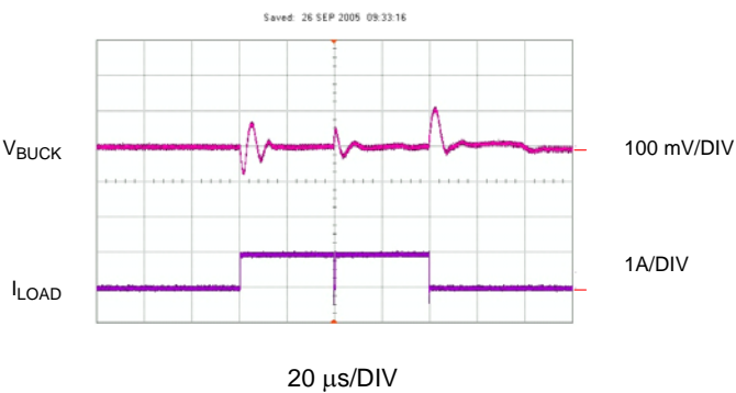
Figure 33: Double-Pulsed Load Response
