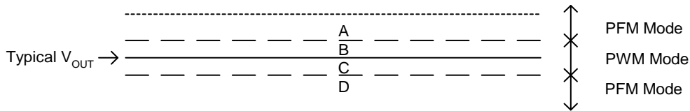
Figure 4: Output Voltage Window
