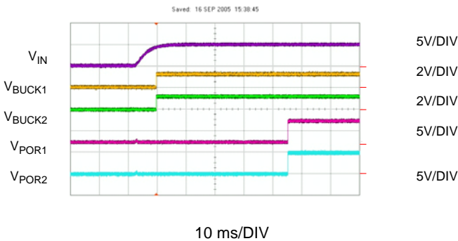
Figure 18: Startup Sequence
