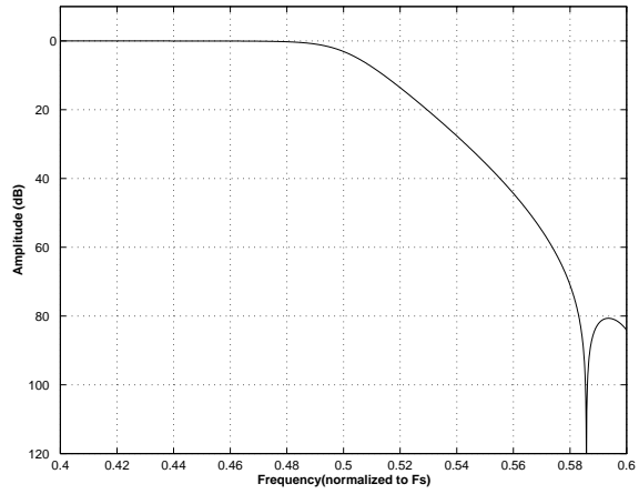
Figure 30. DAC Double Speed (fast) Transition Band
