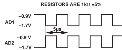
Burn-In Circuit
