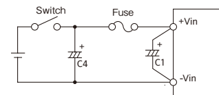
Fig.1-2: Input filter (C4) with Switch
