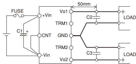
Fig.1-1: Basic Connection
