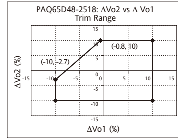
Fig.3-1: PAQ65D48 Standard Model Trim Range
