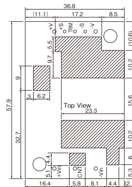
Fig.2-1 Prohibition area of wiring pattern
