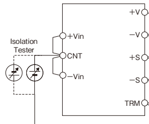
Fig.20-1 Isolation test
