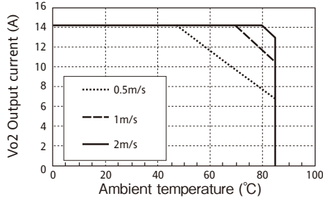
Fig. 1-2 : PAQ65D48-5033 Output Derating
