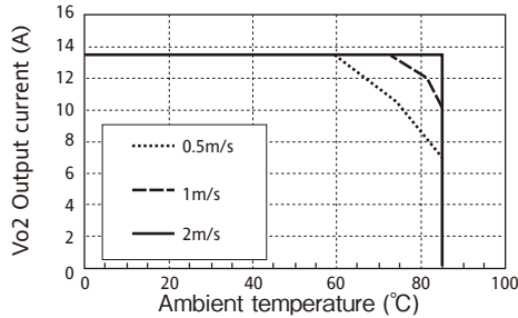
Fig. 1-3 : PAQ65D48-3325 Output Derating
