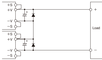
Fig.12-1 Series Operation for High Output Voltage Application
