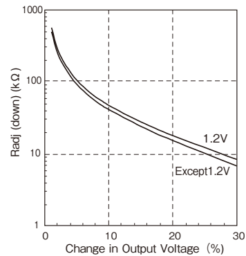
Fig.2-3 Δ(%) vs. R adj (down)
