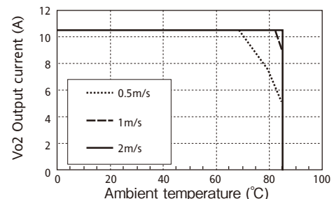
Fig. 1-8 : PAQ65D48-3318 Output Derating
