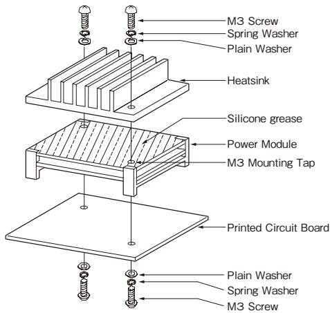
Fig2-1. Installation of Printed Circuit Board and Heatsink
