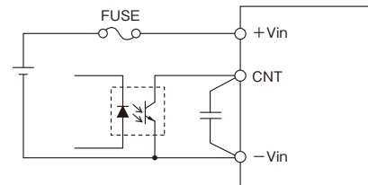
Fig.10-1 : CNT connection
