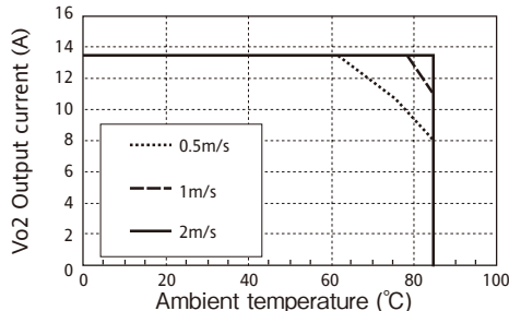
Fig. 1-4 : PAQ65D48-3318 Output Derating
