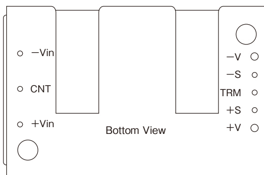
Input and Output Terminal Configurations (Bottom View)
