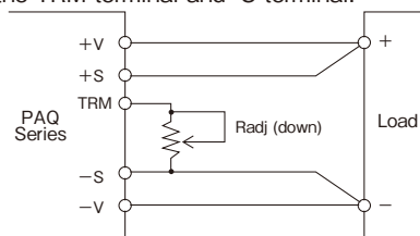
Fig.2-2 Connection for output voltage trim down
