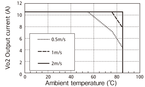
Fig. 1-6 : PAQ65D48-5033 Output Derating
