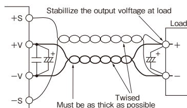
Fig.9-1 Remote Sensing in Use
