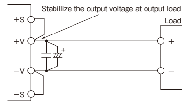
Fig.9-2 Remote Sensing Not in Use (Local Sensing)
