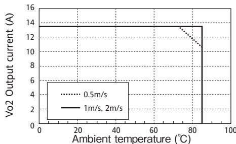
Fig. 1-5 : PAQ65D48-2518 Output Derating
