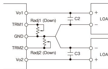
Fig.3-3: Connection for output voltage trim down
