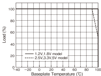
Fig.1-1 PAQ100S48/B Output Derating
