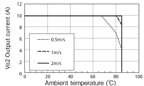
Fig. 1-7 : PAQ65D48-3325 Output Derating
