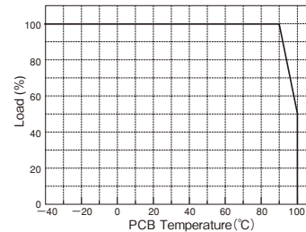
Fig.1-14 Output Derating by PAQ50S48 PCB Temperature
