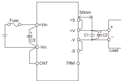
Fig.1-2 Basic Connection
