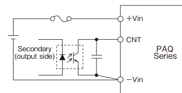
Fig.10-1 CNT connection
