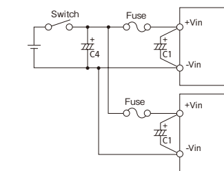
Fig.1-3: Input Filter with Switch when Multiple Power Modules are used.
