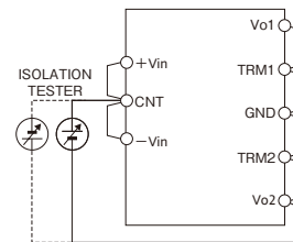
Fig.18-1: Isolation test
