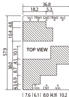
Fig.2-1 : Prohibition area of wiring pattern
