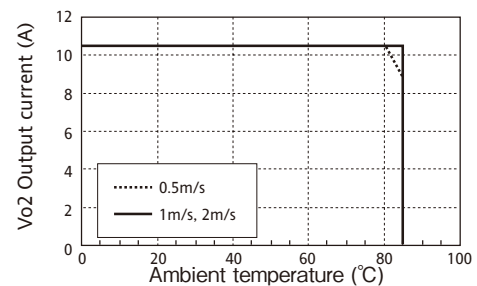
Fig. 1-9 : PAQ65D48-2518 Output Derating
