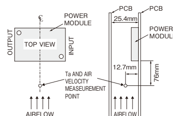
Fig.1-1: Mounting method
