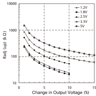
Fig.2-5 \Delta (%) vs. Radj (up)
