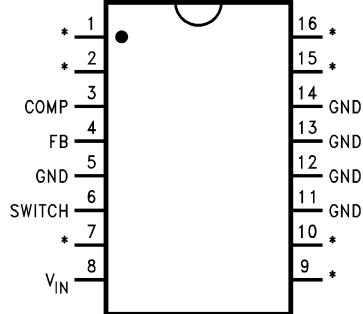
16-Lead DIP (N)
