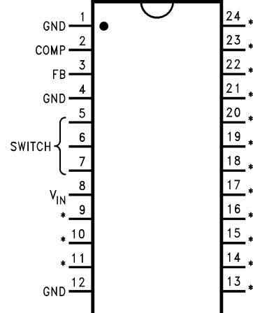
24-Lead Surface Mount (M)
