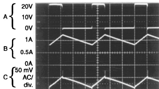
Continuous Mode Switching Waveforms V_{IN} = 20V , V_{OUT} = 5V , I_{LOAD} = 1A L = 52 \mu H , C_{OUT} = 100 \mu F , C_{OUT} ESR = 100 m\Omega
