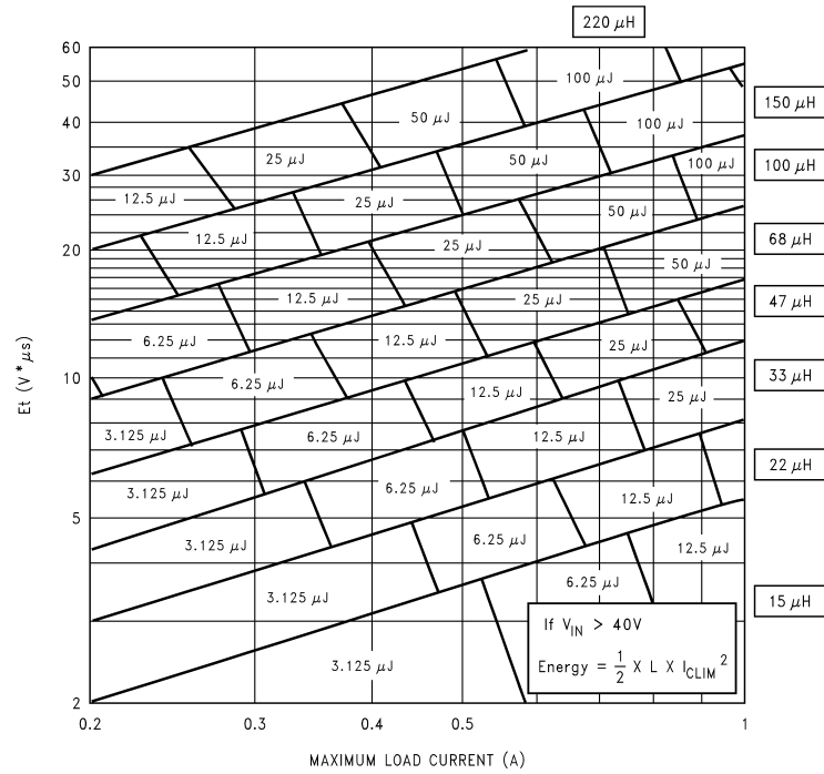
FIGURE 4. LM2591HV-ADJ
