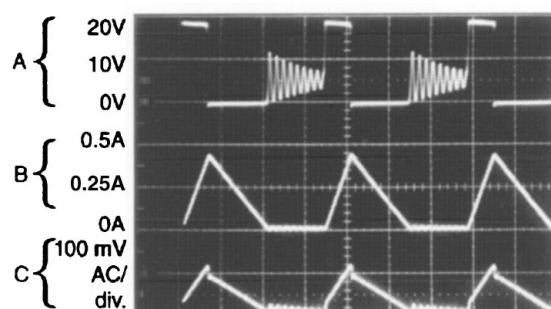
Discontinuous Mode Switching Waveforms V_{IN} = 20V , V_{OUT} = 5V , I_{LOAD} = 250 mA L = 15 \mu H , C_{OUT} = 150 \mu F , C_{OUT} ESR = 90 m\Omega
