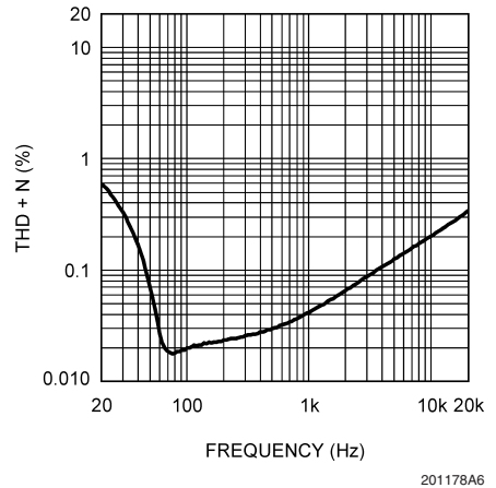
THD+N vs Frequency V_{DD} = 5V, R_L = 8\Omega, A_{V-BTL} = 2V/V P_{OUT} = 1W/Channel, 80kHz BW
