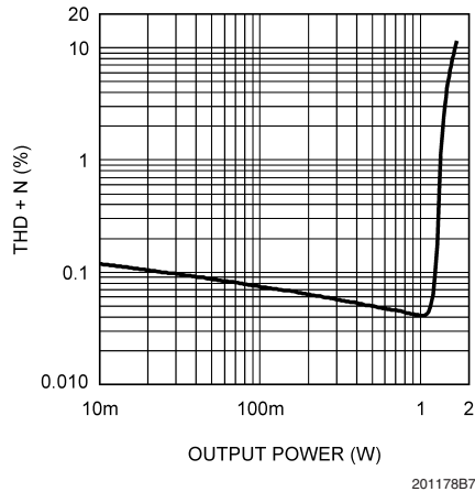
THD+N vs Output Power/Channel V_{DD} = 5V, R_L = 8\Omega, A_{V-BTL} = 2V/V f = 1kHz, 80kHz BW
