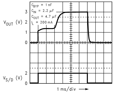
Turn-On Time (LP2988)
