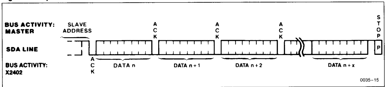
Figure 9: Sequential Read
