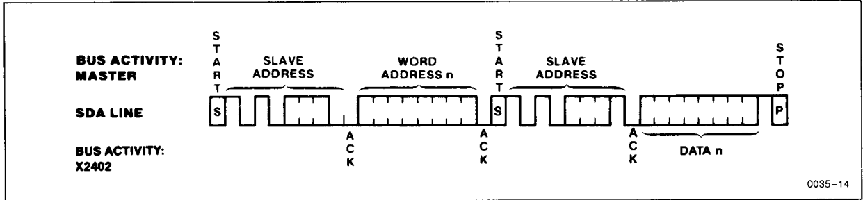
Figure 8: Random Read
