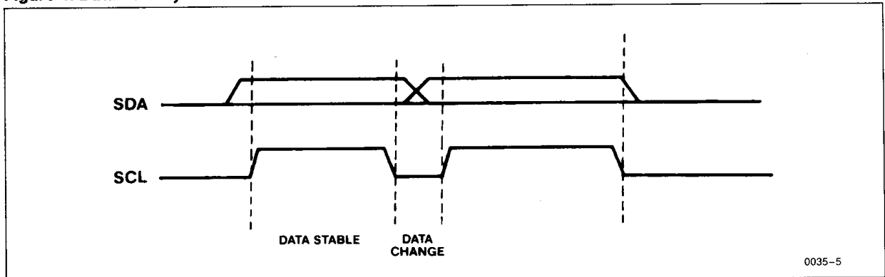
Figure 1: Data Validity
