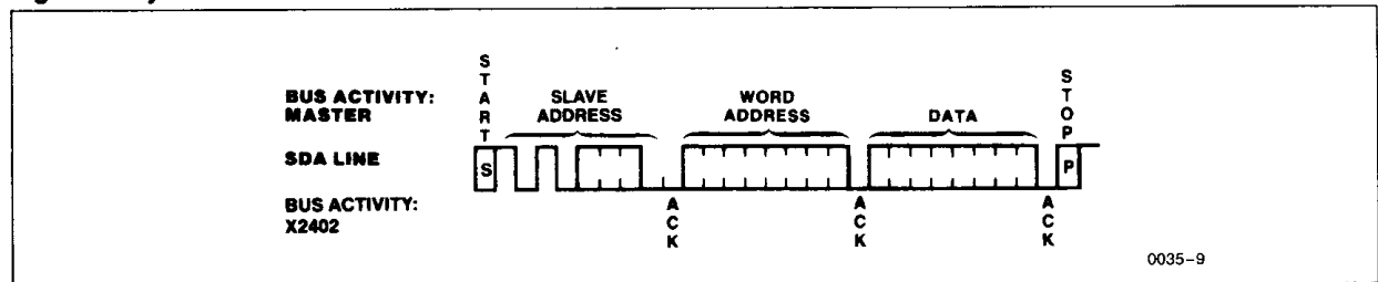
Figure 5: Byte Write
