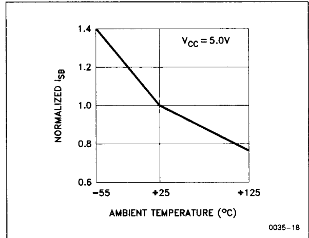
Normalized Standby Supply Current vs. Ambient Temperature
