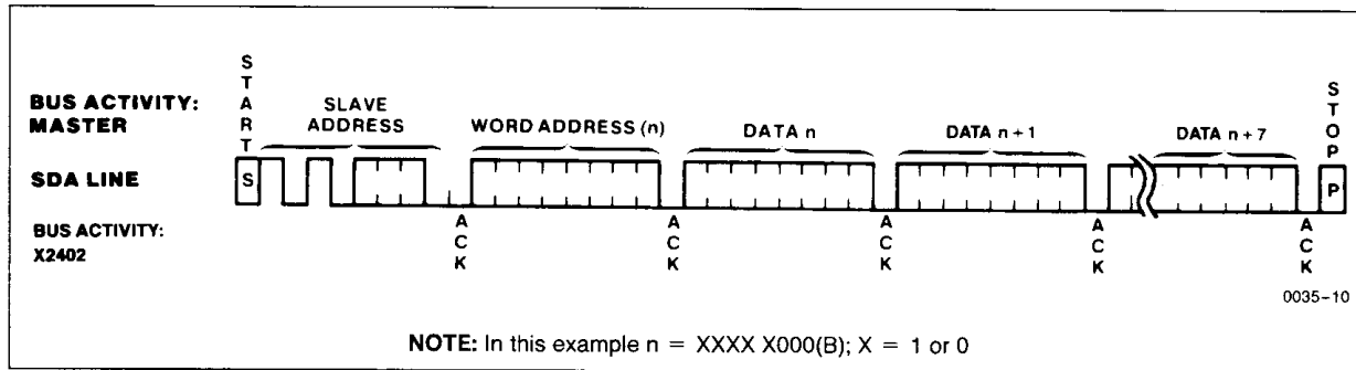
Figure 6: Page Write
