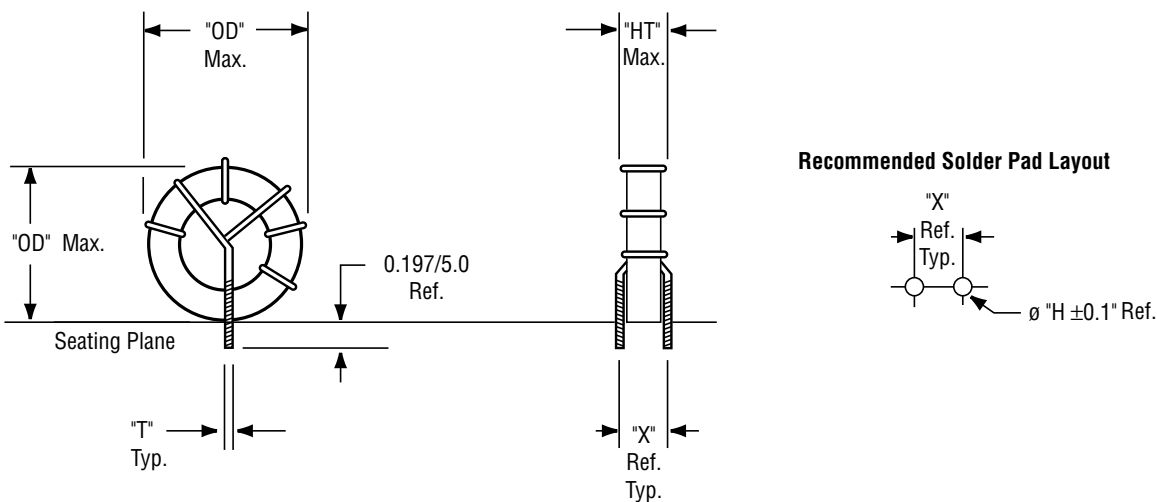
Figure 1 - Vertical Mount
