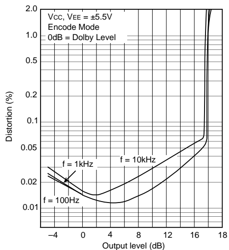
NR off total harmonic distortion
