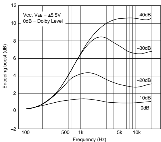
NR B type encoding characteristics
