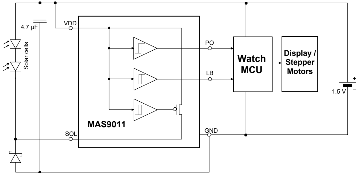
Figure 1. Typical application circuit of MAS9011
