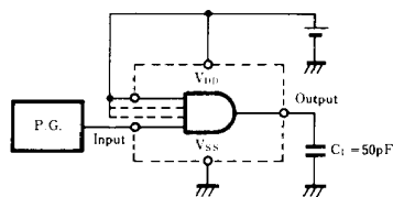
1. Switching Time Test Circuit
