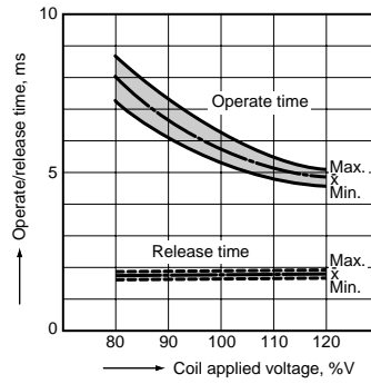
3-(4). Operate/release time Sample: JW2aSN-DC24V, 6 pcs. Ambient temperature: 20°C 68°F
