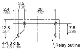
PC board pattern (Copper-side view)
