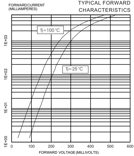
FIG. 10 (For CDBA140SL)
