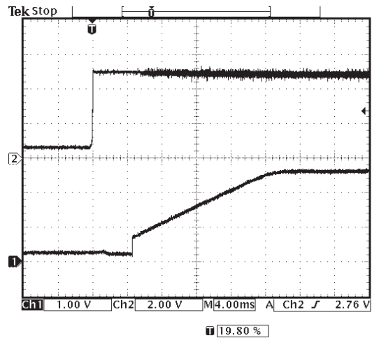
Figure 30: Typical Power-up Characteristic (Channel 1: V_o , Channel 2: V_{in} )
