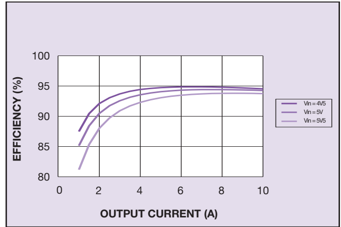
Figure 26: Efficiency vs Load
