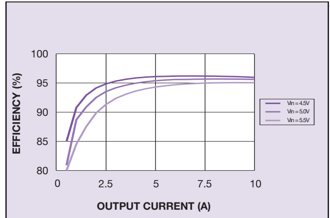
Figure 42: Efficiency vs Load
