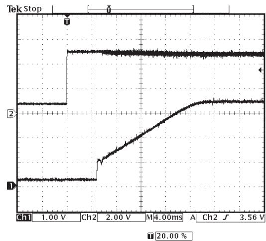
Figure 46: Typical Power-up Characteristic (Channel 1: Vo, Channel 2: Vin)
