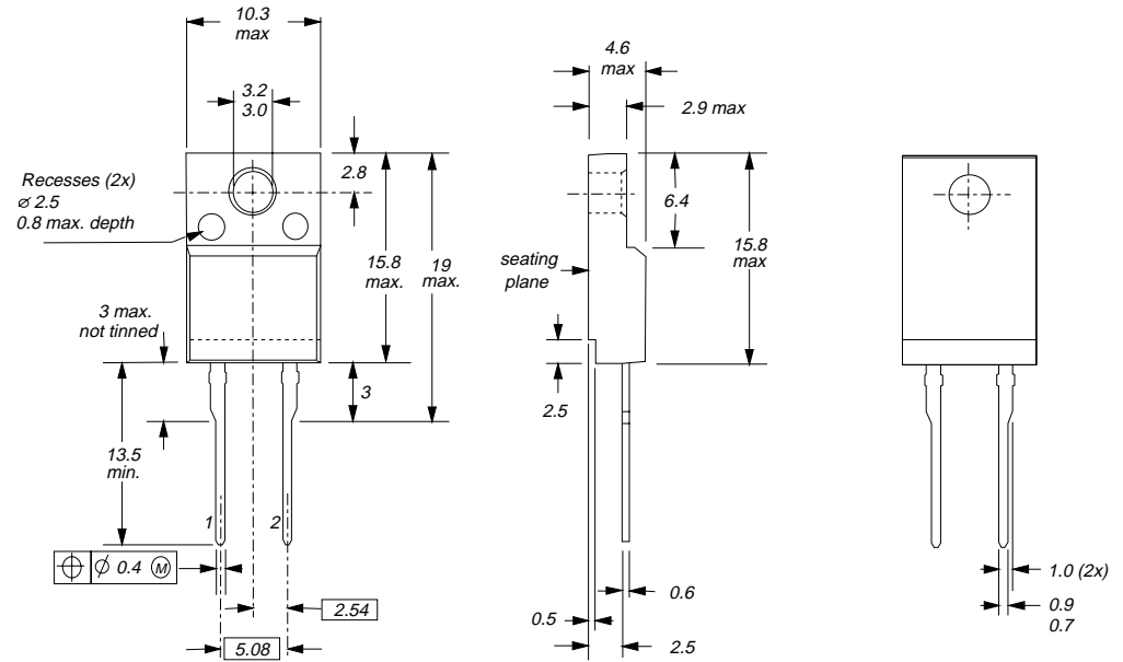
Fig.11. SOD113; The seating plane is electrically isolated from all terminals.
