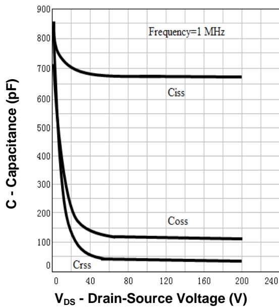
Capacitance
