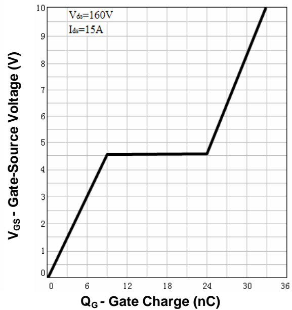
Gate Charge
